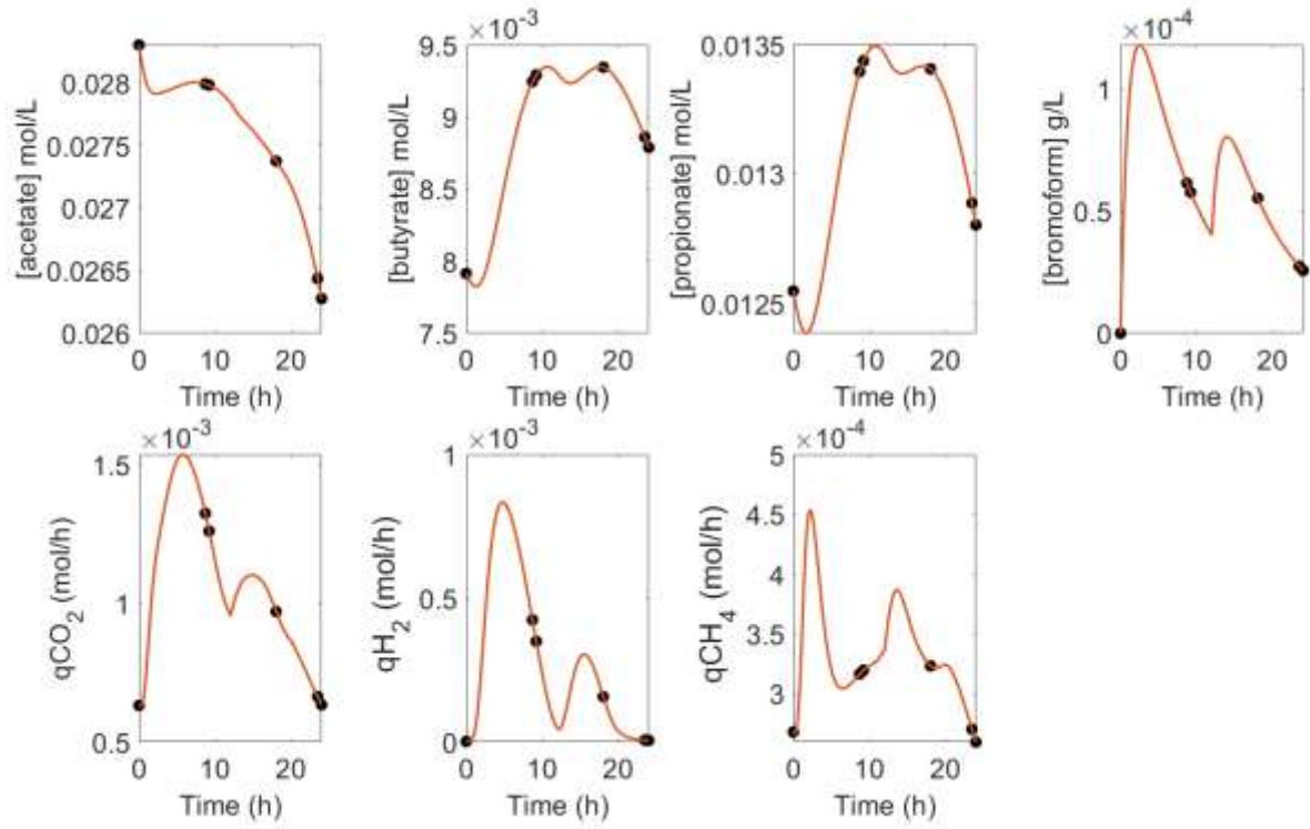
590 Fig. 4. Theoretical dynamic response of the model variables under the Optimal 591 Experiment Design conditions for two feed distributions at 70% and 30% of the total 592 DM ( n_r = 2 , \omega_1 = 0.7 ; \omega_2 = 0.3 ). The circles • are the optimal sampling times.
