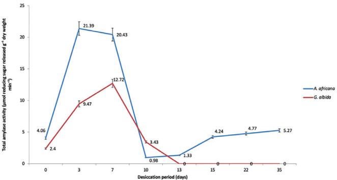
Figure 5. Total amylase activity ( \mu\text{mol} reducing sugar released \text{g}^{-1} dry weight \text{min}^{-1} ) in seeds of A. africana and G. albida following desiccation; error bars indicate variability at p \leq 0.05 . A. africana = Azelia africana ; G. albida = Gambeya albida .
