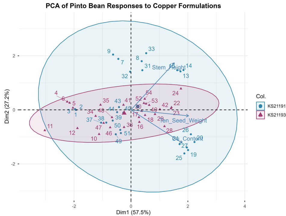
Figure 5. PCA biplot illustrating the clustering of treatments based on all measured growth, yield, and seed quality variables.
