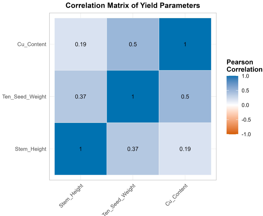
Figure 6. Correlation matrix (heatmap) showing Pearson's correlation coefficients between measured parameters across all treatments and cultivars.
