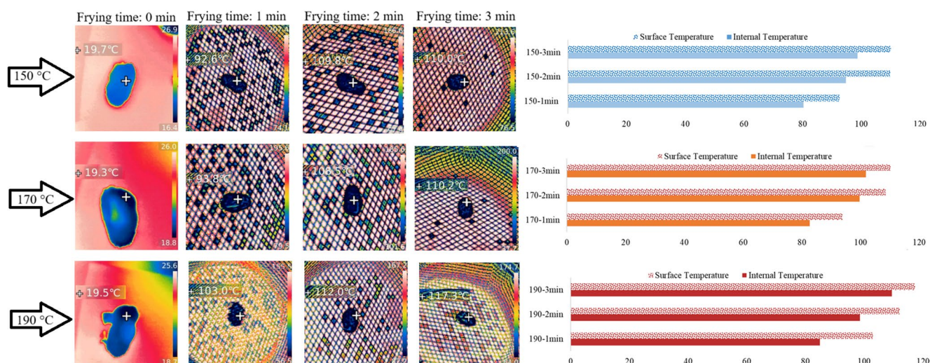
Fig. 1 Real-time thermal evolution of oleaster seed flour (OSF)-coated mussels during deep-fat frying at different temperatures (150, 170, and 190 °C): Infrared thermography images (left) and surface/core temperature profiles (right)
