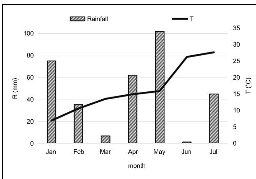
Figure 3. Trend of the total monthly rainfall ( R ) and the mean air temperature ( T ) from January to July 2019 (Data provided by the Lazio Regional Agency for Development and Agricultural Innovation Meteorological Station of Rome, Lanciani Street).
