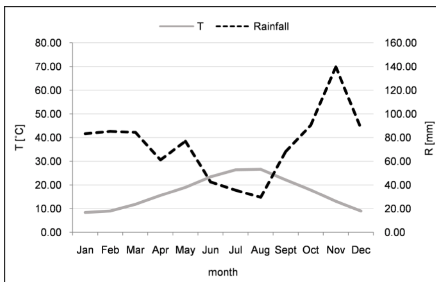
Figure 2. Climatic diagram according to Bagnouls and Gaussen (1953), for the period 2008-2018. The mean monthly air temperature ( T^{\circ} ) and the total monthly rainfall ( R ) are shown. The area between the two curves shows the period of summer drought. (Data provided by the Lazio Regional Agency for Development and Agricultural Innovation Meteorological Station of Rome, Lanciani Street).
