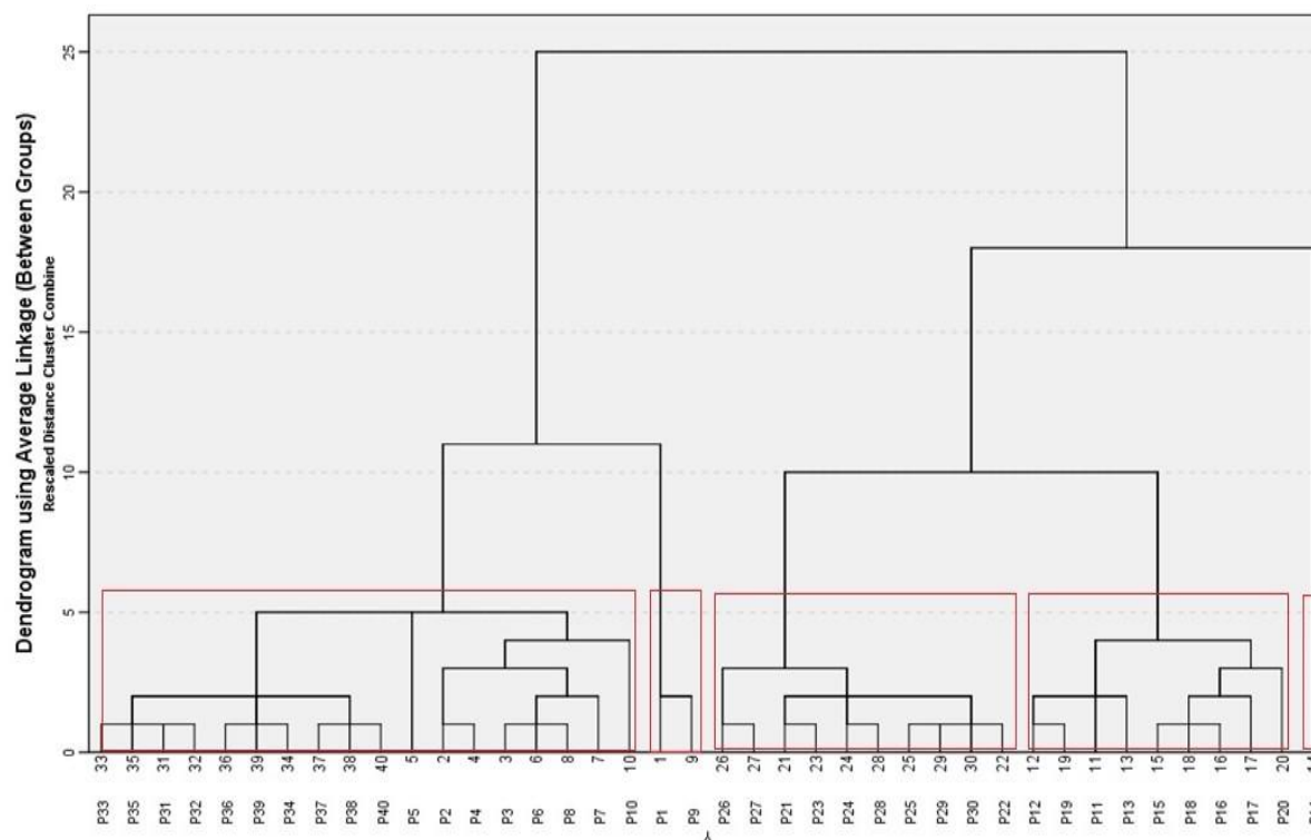
Fig. 1. Dendrogram depicting genetic relationships amongst 40 populations of Acorus calamus in wetlands of Kashmir valley
