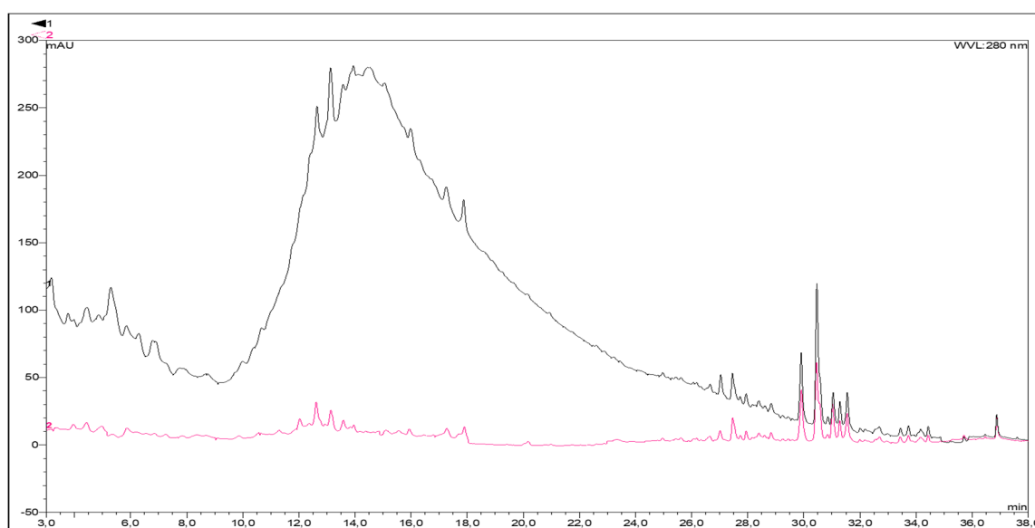
Figure 4. Results of high-performance liquid chromatography UV diode-array detection (HPLC-DAD) at 280 nm of fraction F (black curve) and Sf (red curve) at a concentration of 2 g/L. Compounds were separated in a Kinetex F5 analytical column; mobile phase was methanol and water in 0.1% formic acid, gradient elution, at 35 °C. Chromatographic conditions are reported in Section 4.7.
