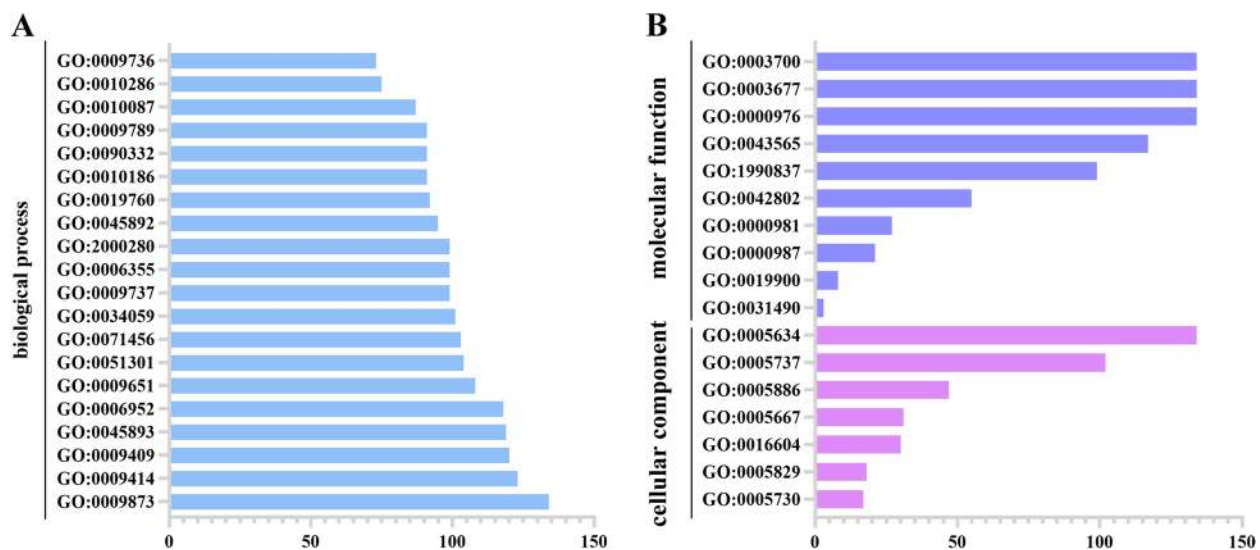
Fig. 3 Gene Ontology (GO) results in TkAP2/ERF proteins. Different colored represent different function
