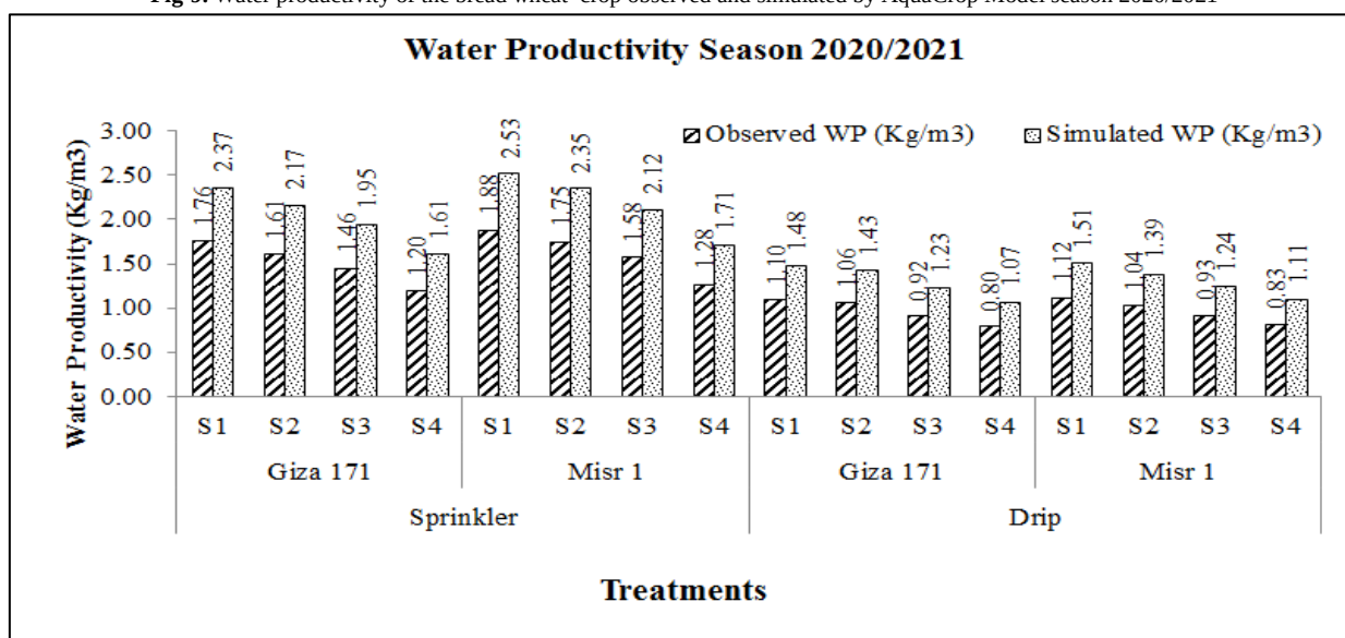
Fig-9. Water productivity of the bread wheat crop observed and simulated by AquaCrop Model season 2020/2021
