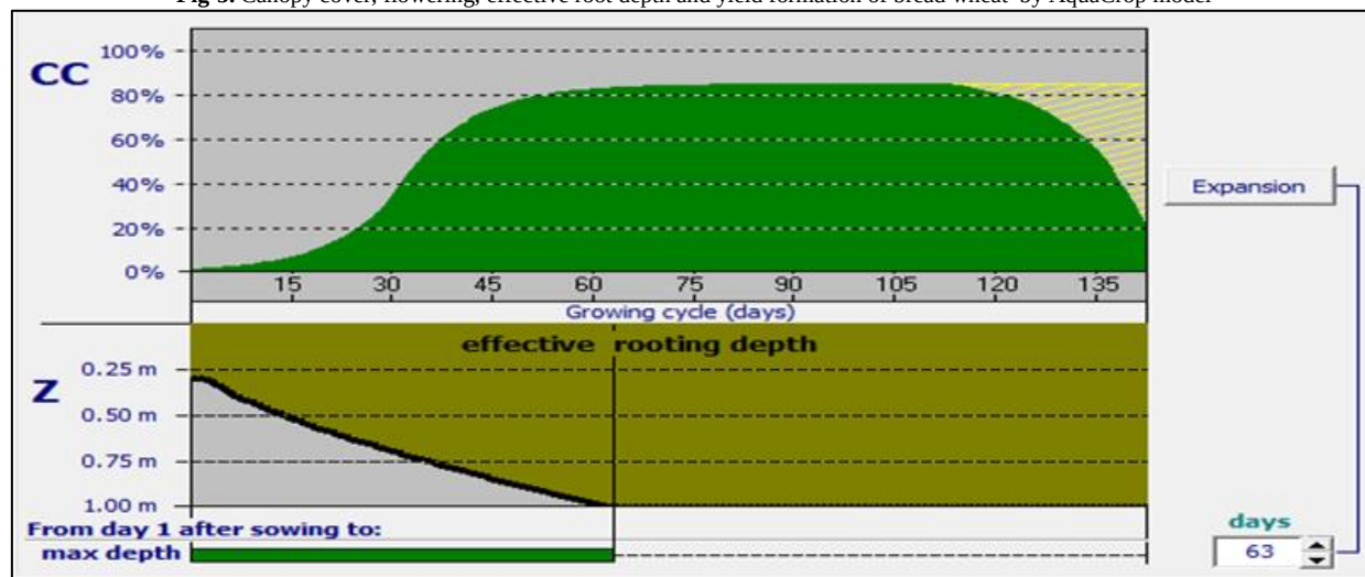
Fig-5. Canopy cover, flowering, effective root depth and yield formation of bread wheat by AquaCrop model
