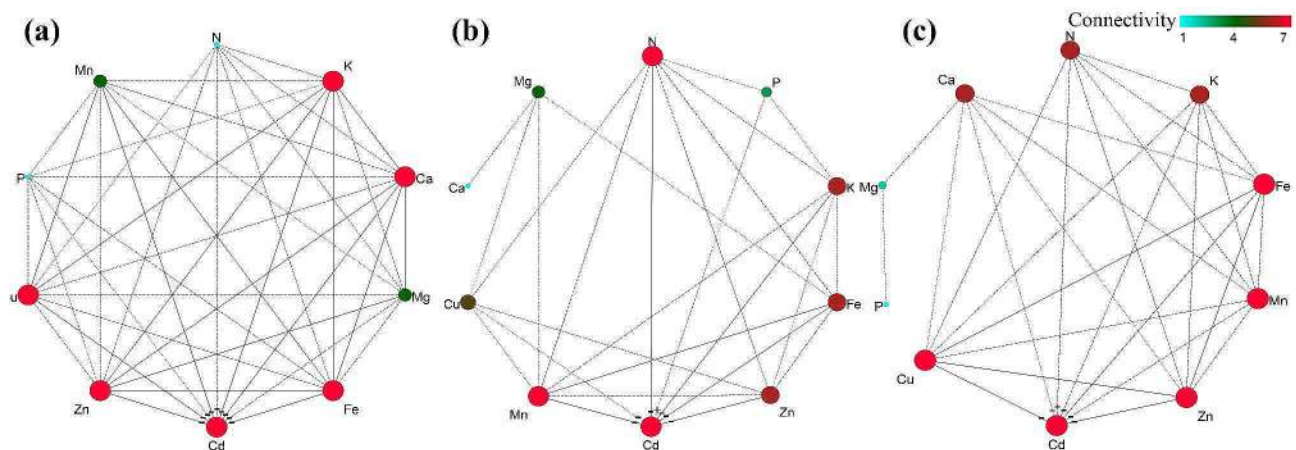
Fig. 3 The interaction network analysis of mineral elements in S. nigrum roots (a) , stems (b) and leaves (c) under Cd concentrations treatments. The redder the node color and the larger the circular node in the weight network analysis, the greater the element's connectivity in the weight network, that is, the more distinct the influence of this element on other nutrient elements. The different lines between the mineral elements (dotted and solid) represent the degree of correlation. "+" represents there is a positive correlation between the two elements, and "-" represents there is a negative correlation between the two elements
