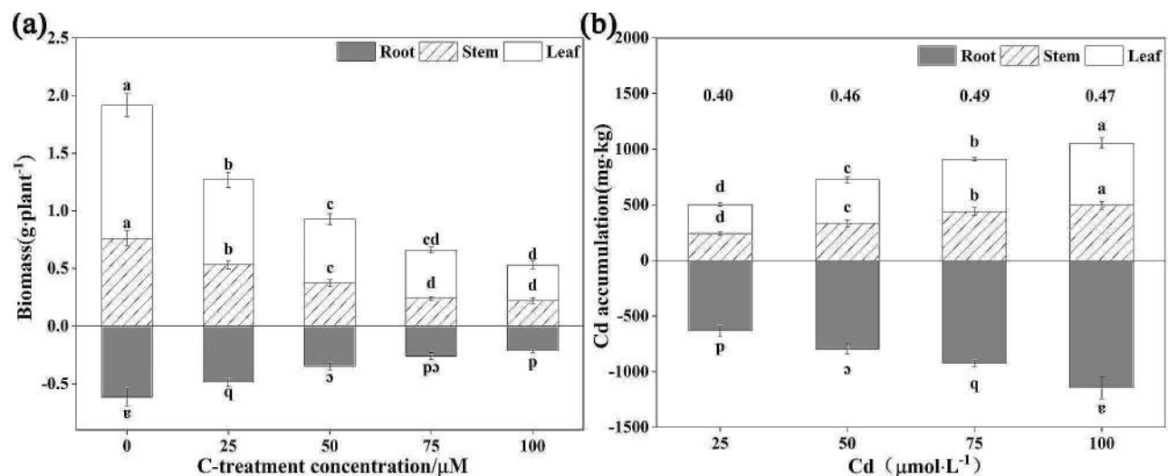
Fig. 1 The influences of different Cd treatment on biomass growth (a) and Cd accumulation (b) in S. nigrum . The number at the top of the bar chart shows the TF value of Cd in S. nigrum (b) . The values are the mean \pm SD ( n = 3 ). Different lowercase letters labeled on the columns show significant differences between different Cd treatments using Tukey's test ( P < 0.05 )
