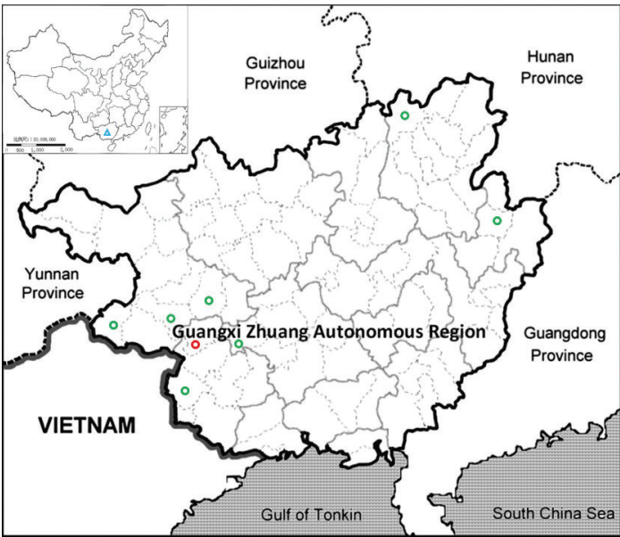
Figure 5. The distribution of Justicia tiandengensis Y.Nong & G.Y. Wei (red circle) and J. leptostachya Hemsl. (green circle) in Guangxi (blue triangle), China.
