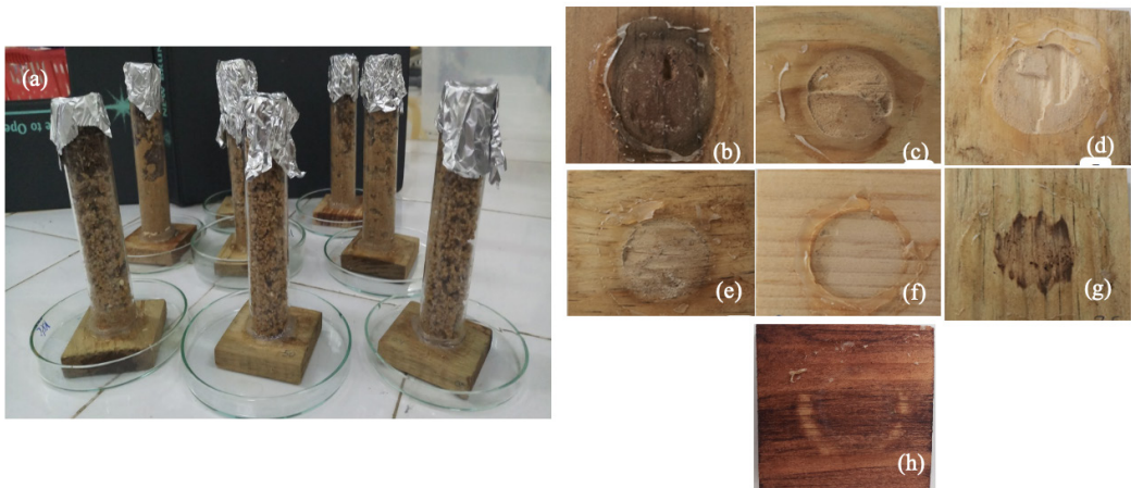
Figure 5: Photographs of pinewood samples exposed to biodeterioration with termites. a) Arrangement of wood blocks for EN 118:2013 (2013) test, b - h) The attacked pinewood species by Coptatermes Curvig-nathus were impregnated with CuNPs at concentrations of control negative; 1 mg/ml; 2 mg/ml; 3 mg/ml; 4,5 mg/ml; 6 mg/ml and control positive.
