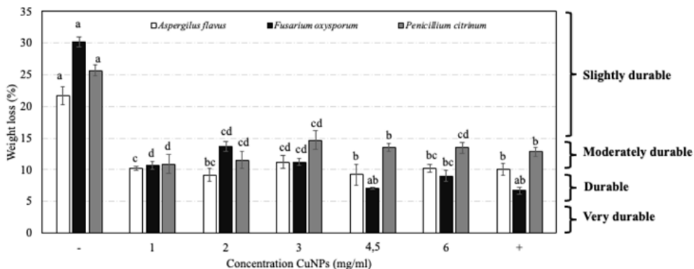
Figure 4: The figure antifungal activity at all concentrations of CuNPs (control negative; 1 mg/ml; 2 mg/ml; 3 mg/ml; 4,5 mg/ml; 6mg/ml, and control positive) with 3 fungal trains: A. flavus , F. oxysporum , and P. citrinum according to EN 113-2:2020 (2020). The letters abcd represent statistically significant differences in each other fungal strain of the Duncan test, P < 0,05.
