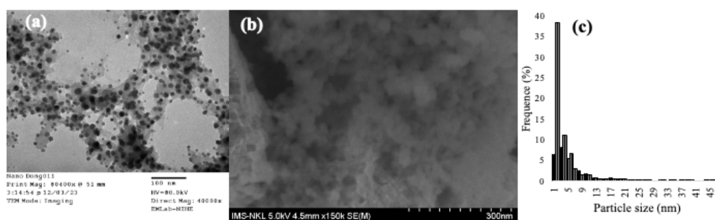
Figure 2: Biologically synthesized CuNPs using Cleistocalyx operculatus leaf extract. (a) TEM, (b) SEM, (c) histogram of CuNPs size distribution.
