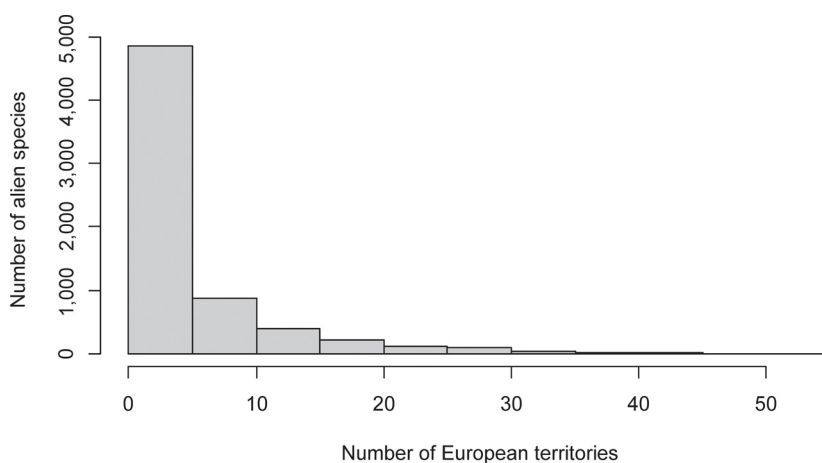
Fig. 5. Frequency of occurrence of 7,335 alien plant species in European territories ( n = 55 ).
