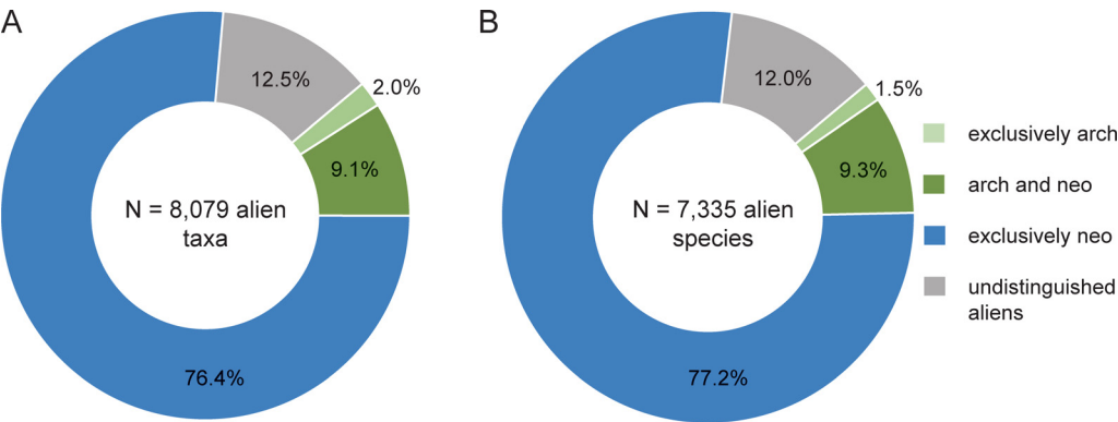
Fig. 1. Proportions of (A) alien plants (all taxa) and (B) alien plants at the species level in categories of residence time in the European alien flora. Exclusively arch – taxa or species listed exclusively as archaeophytes across Europe; arch and neo – taxa or species listed as archaeophytes for one part and as neophytes in another part of Europe; exclusively neo – taxa or species listed exclusively as neophytes in Europe; undistinguished aliens (arch+nat) – taxa or species listed as aliens without residence time indication or listed as archaeophyte or neophyte only for a part of Europe and as alien in another part. Additional 57 taxa (43 species) with uncertain alien status in Europe were excluded.
