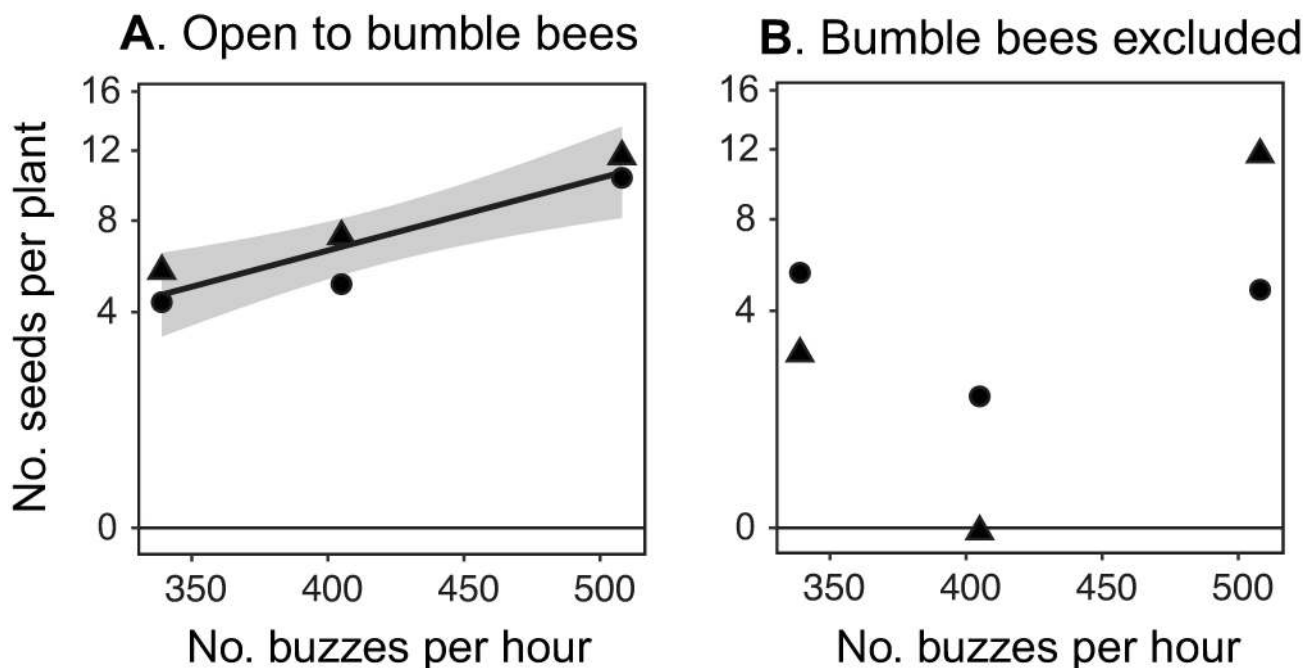
Fig 5. Acoustic surveys predict pollination services in two alpine flowering forbs. When flowers of Trifolium dasyphyllum (circles) and T. parryi (triangles) are left open to bumble bee visitors, buzz abundance (A) predicts the average number of seeds per plant in each of three 0.01 km 2 plots. When bumble bee pollinators are excluded, buzz abundance fails to predict seed set (B), illustrating that acoustic surveys document pollination services by bumble bees. Gray shading around the line represents the standard error of the mean [47].
