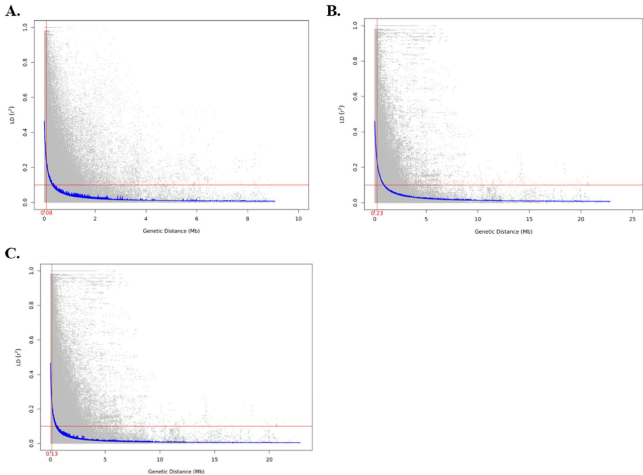
Fig. 5 Scatter plot of linkage disequilibrium (LD) decay, showing mean r^2 values plotted against physical distances between markers (Mb) A A-subgenome B C-subgenome C Whole genome. The blue curve illustrates the LD decay pattern modelled using a smoothing spline regression. The vertical red line shows the position where the decay curve meets the half-decay threshold at r^2=0.2 . The horizontal red line marks the genome-wide half-decay r^2 value
