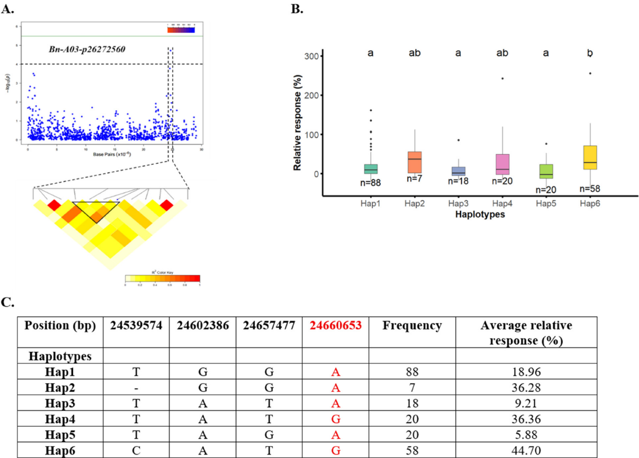
Fig. 7 GWAS results and haplotype analysis for SNP Bn-A03-p26272560 associated with RR-RE. A A Manhattan plot illustrating RR-RE is shown. The green and black horizontal lines mark the Bonferroni & suggestive significance threshold, respectively. Linkage disequilibrium (LD) among SNPs on chromosome A03 is displayed below, based on pairwise r^2 values, which are color-coded according to the provided scale. B Phenotypic differences in osmopriming response (RR-RE) between the identified haplotypes C Haplotype analysis of SNP Bn-A03-p26272560 (in red text) and three other linked SNPs. Six haplotypes (Hap1, Hap2, Hap3, Hap4, Hap5 and Hap6) were identified in 211 accessions
