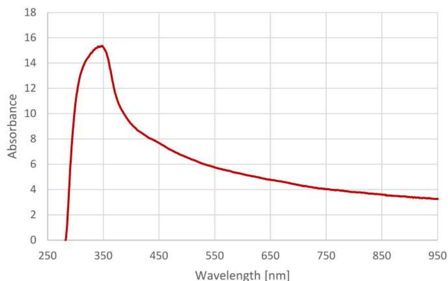
Figure 3. The UV-Vis spectrum of ZnO NPs biosynthesized from C. glomerata extract.
