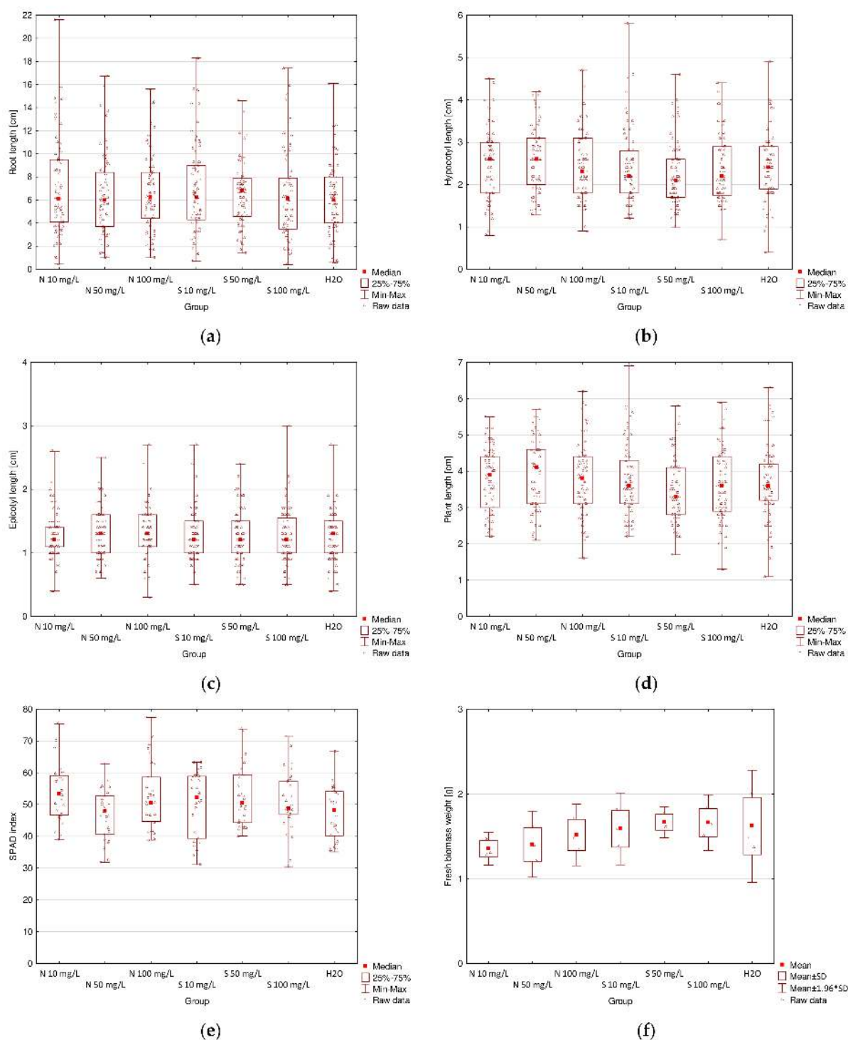
Figure 5. Box plots for results of germination tests with the use of various concentrations of ZnO NPs and ZnSO 4 : (a) root length; (b) hypocotyl length; (c) epicotyl length; (d) whole plant length; (e) chlorophyll content; (f) fresh biomass weight.
