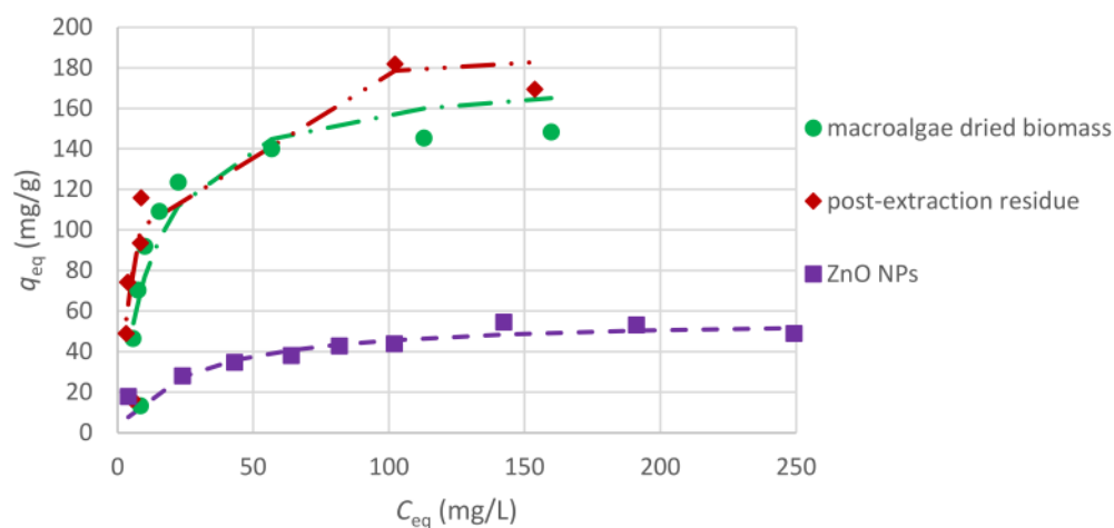
Figure 9. Adsorption isotherms for different sorbents ( C_0 of 25–300 mg/L and C_S of 10 g/L, and pH of 5).
