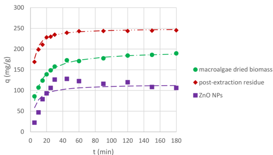
Figure 8. Effects of sorbent type on Cr(III) ion sorption capacity (pH of 5; C_S , 1 g/L; and C_0 , 300 mg/L).
