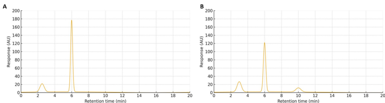
Fig. 2 Representative HPLC chromatograms. Glabridin standard showing the characteristic peak at t_R \approx 6.0 min (A) and G. glabra extract chromatogram displaying the corresponding glabridin peak (B)
