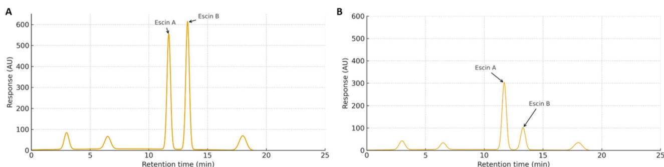
Fig. 1 Representative HPLC chromatograms. Escin standard showing two major saponin peaks (Escin A and Escin B) (A) and A. hippocastanum extract chromatogram displaying corresponding saponin peaks (B)
