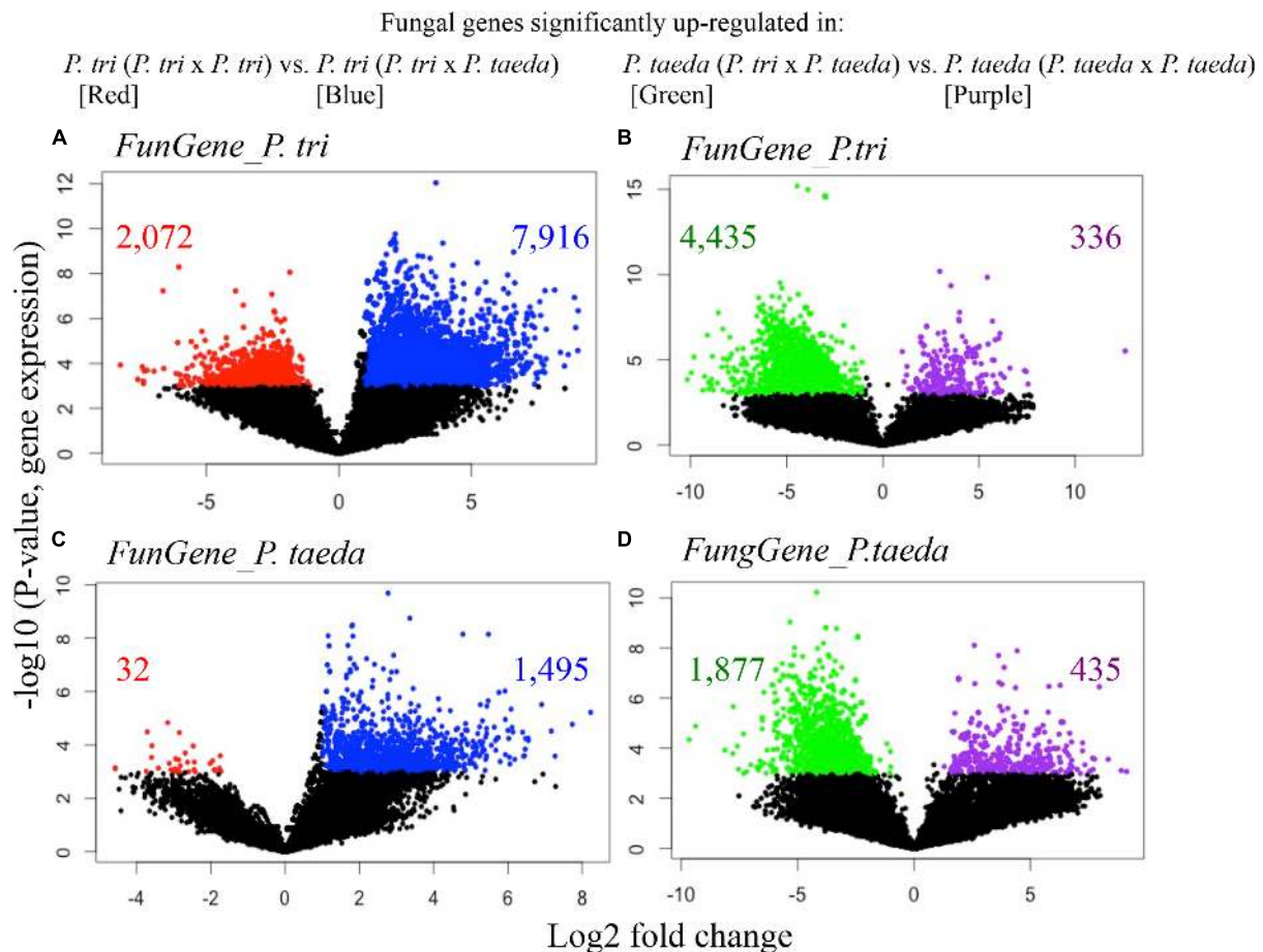
FIGURE 5 | Volcano plots show the expression of fungal genes originally expressed in Populus trichocarpa roots ( FunGene_P. tri , A,B ) in Pinus taeda roots ( FunGene_P. taeda , C,D ) in response to neighbor plant species. (A) FunGene_P. tri on P. trichocarpa roots that were up-regulated (in blue) or down-regulated (in red) when grown with P. taeda compared to with P. trichocarpa ; (B) FunGene_P. tri on P. taeda roots that were up-regulated (in green) or down-regulated (in purple) when P. taeda was grown with P. trichocarpa compared to with P. taeda . (C) FunGene_P. taeda on P. trichocarpa roots that were up-regulated (in blue) or down-regulated (in red) when grown with P. taeda compared to when grown with P. trichocarpa ; (D) FunGene_P. taeda on P. taeda roots that were up-regulated (in green) or down-regulated (in purple) when P. taeda was grown with P. trichocarpa compared to when grown with P. taeda . Data of loading gene factors were generated using coordinate scales on the left (log10 of expression rate) and the bottom (mean of log2-fold changes). Cross-comparative expression of the genes was analyzed using t -test to compare the fungal genes of the roots from a plant species grown with conspecific vs. heterospecific neighbors ( n \geq 3 ; Wilcox.Test P < 0.01 ; FDR < 0.05 ; fold changes \geq 2 ). The total counts of genes detected and significant changes in gene counts in response to neighbor effects are listed in Supplementary Dataset 3 .
