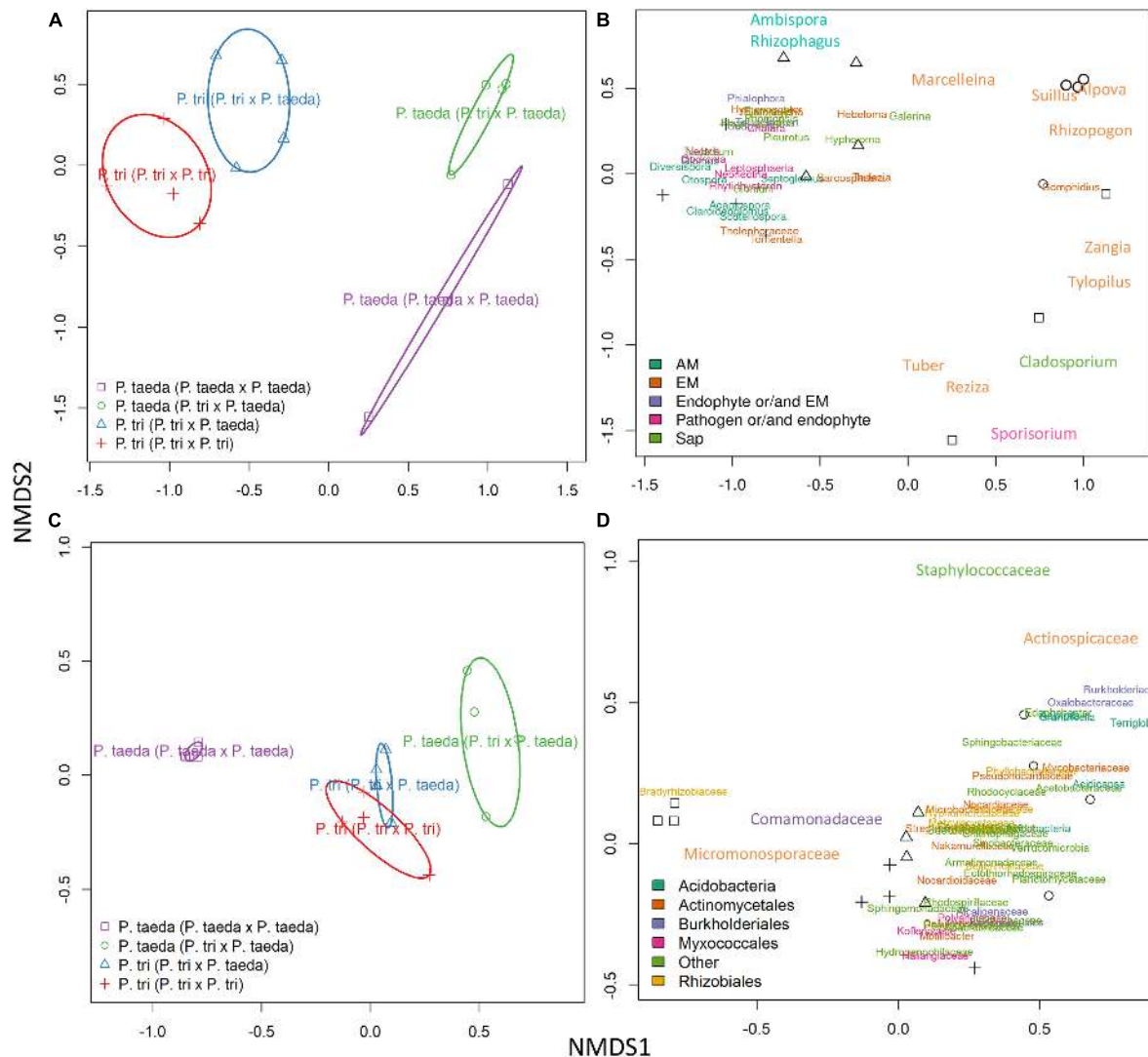
FIGURE 4 | Non-metric multidimensional scaling plots showing the taxonomic composition of different plant host root microbiomes associated with same vs. different neighboring plant species. PERMANOVA was used to determine the changes of fungal (A,B) and bacterial (C,D) taxa associated with neighboring plant species (Supplementary Table 3 and Supplementary Datasets 2B,D). AMF, arbuscular mycorrhizal fungi; EMF, ectomycorrhizal fungi; Sap, Saprotrrophic fungi. The pairwise comparisons were applied to each microbial taxon (Supplementary Datasets 2B,D). P. tri = P. trichocarpa .
