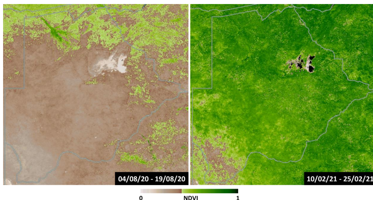
Figure 1 – Normalised Difference Vegetation Index (NDVI) maps of Botswana during the dry season (left) and wet Season (right). Maps are 16-day NDVI averages. Data taken from NASA Worldview (NASA, 2022).
