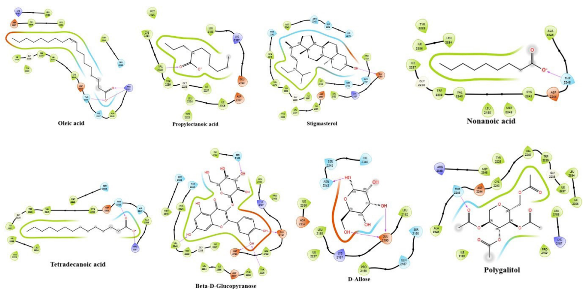
Figure 3. Docking interactions of Ziziphus mauritiana phytochemicals with STAT-3 (PDB ID: 6NJS).
