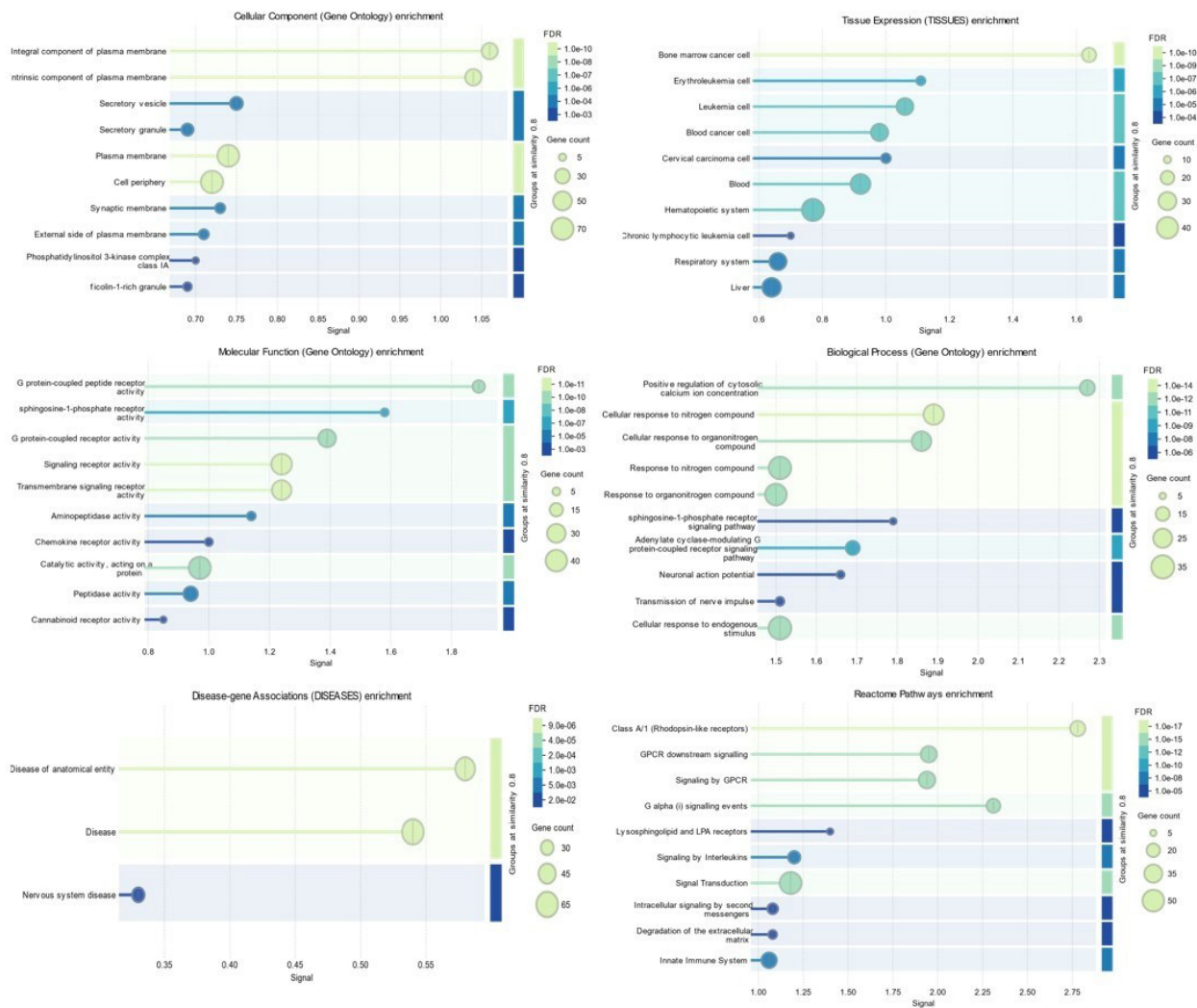
Figure 2. Gene Ontology enrichment analysis of predicted protein targets interacting with phytocompounds from Ziziphus mauritiana seed extract.
