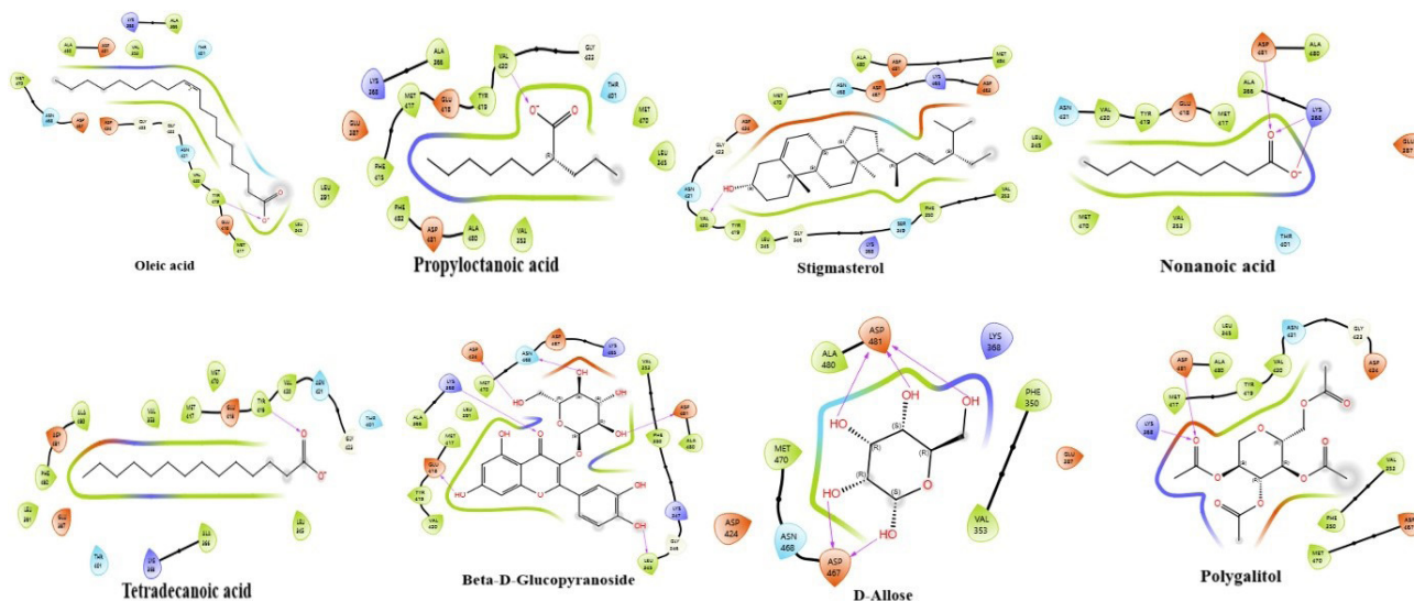
Figure 4. Docking interactions of Ziziphus mauritiana phytochemicals with PI3K gamma (PDB ID: 4RA4).
