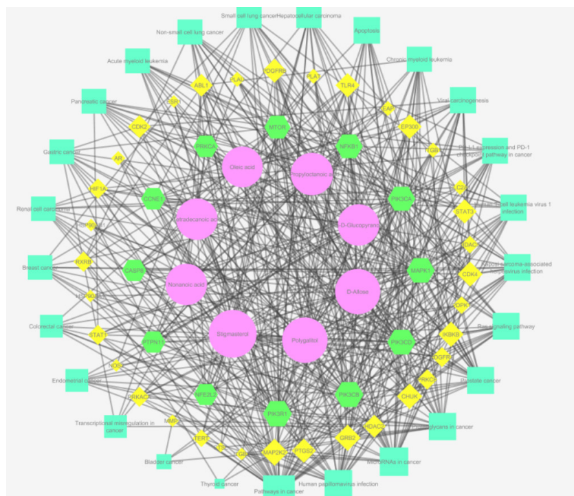
Figure 1. Network representation of molecular pathways and protein targets modulated by the phytochemicals from Ziziphus mauritiana seed extract.
