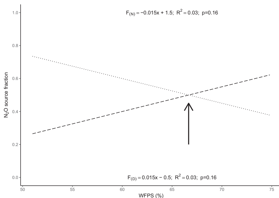
Fig. 4. N_2O source fractions over the observed range of soil WFPS. Dotted line = predicted fraction of nitrification ( F_N ) and dashed line = predicted fraction of denitrification ( F_D ). Arrow = intersection of F_N and F_D .
