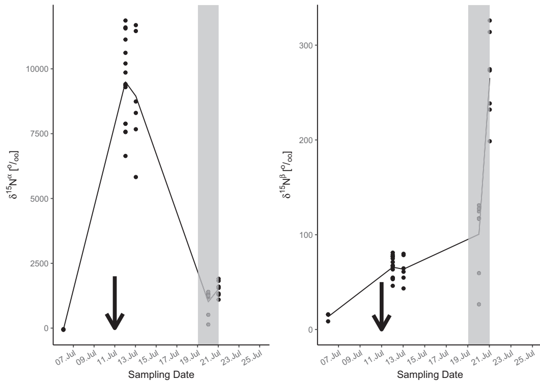
Fig. 2. Temporal plot of \delta^{15}\text{N}^{\alpha} and \delta^{15}\text{N}^{\beta} changes over the sampling period. Solid line = mean \delta^{15}\text{N}^{\alpha} and \delta^{15}\text{N}^{\beta} on each sampling date. Black arrows = ^{15}\text{N} labelled urea fertiliser application; shaded area = heavy rainfall. (See main text for further explanation of large \delta value scales).
