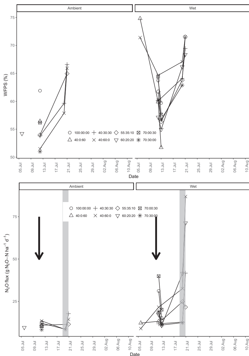
Fig. 1. Temporal plot of soil WFPS and daily \text{N}_2\text{O} fluxes subset data based on Eq. (2) concentration rule (Legend = Mixture Ratio; Black arrows = fertiliser application; shaded area = heavy rainfall). Full dataset presented in Bracken et al. (2020).
