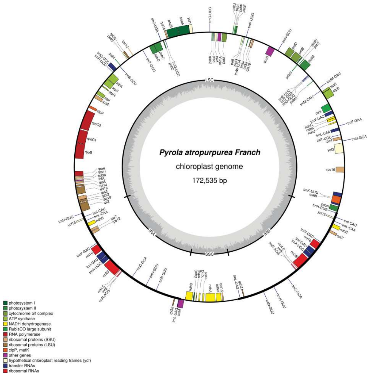
Figure 1: The P. atropurpurea chloroplast genome map in the genus Pyrola
