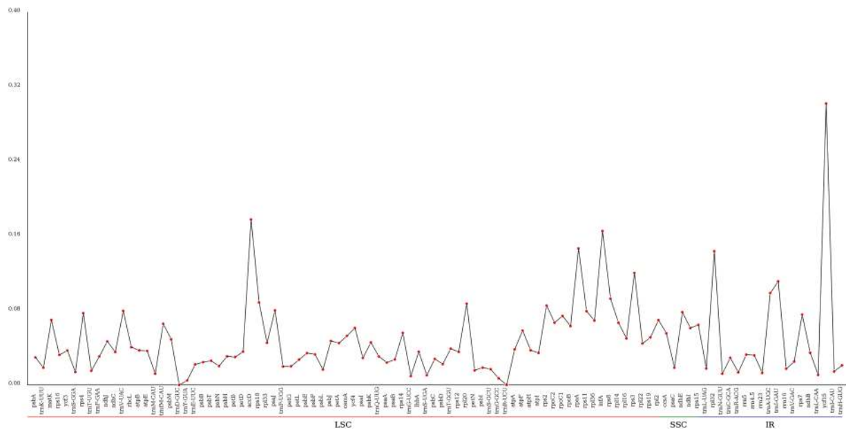
Figure 3: Divergent hot-spot nucleotide sites in Ericaceae species' chloroplast genomes
