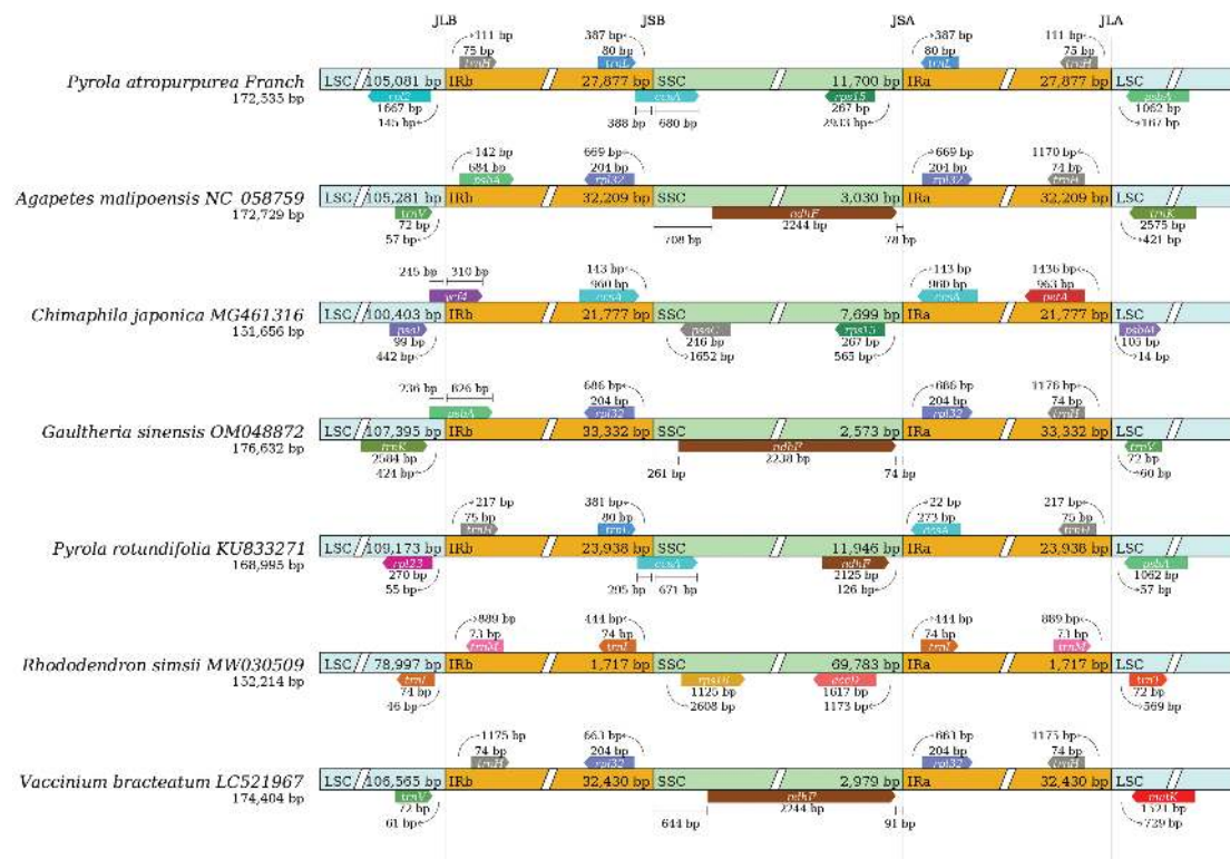
Figure 4: Boundary comparison of Ericaceae chloroplast genome
