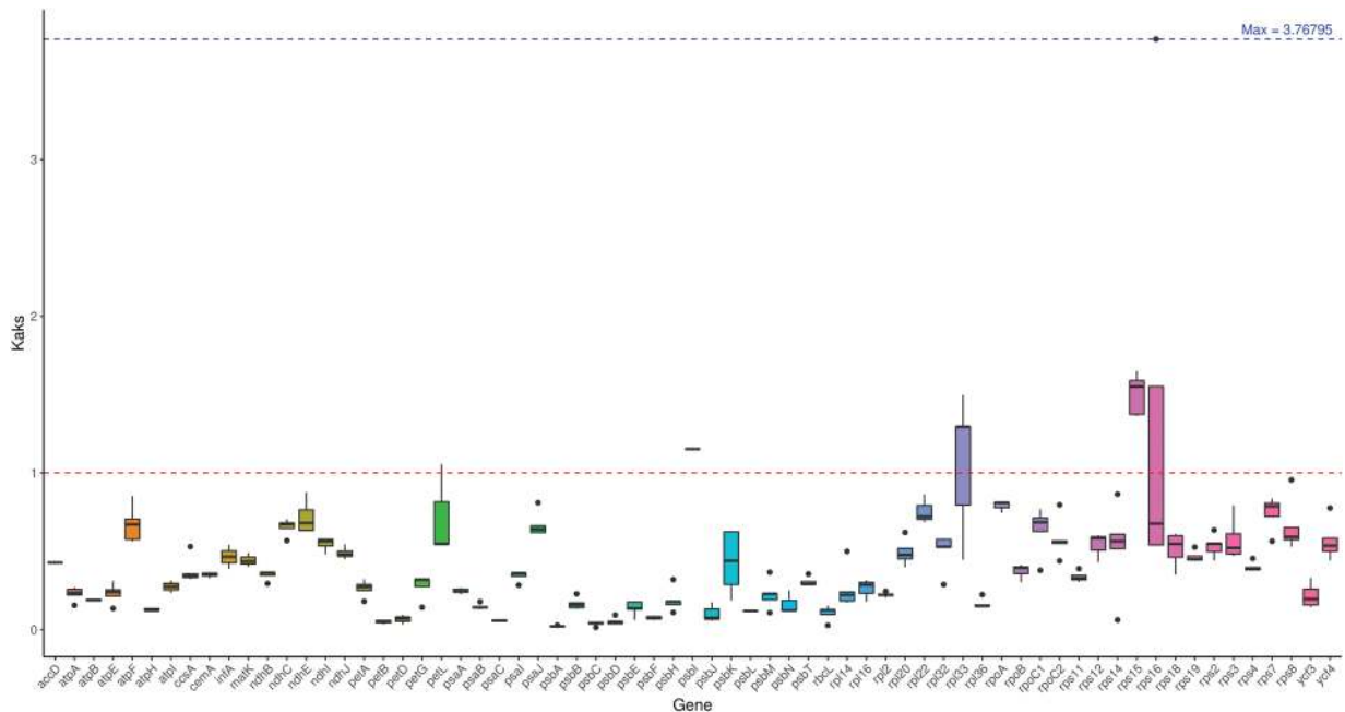
Figure 6: Ka/Ks values of common PCGs in P. atropurpurea
