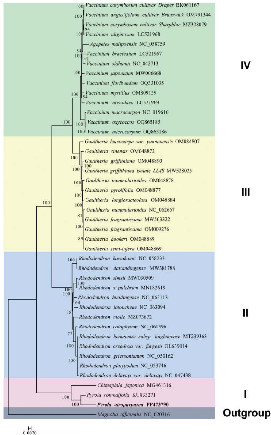
Figure 7: The phylogenetic tree of 41 Ericaceae species based on chloroplast genome PCGs
