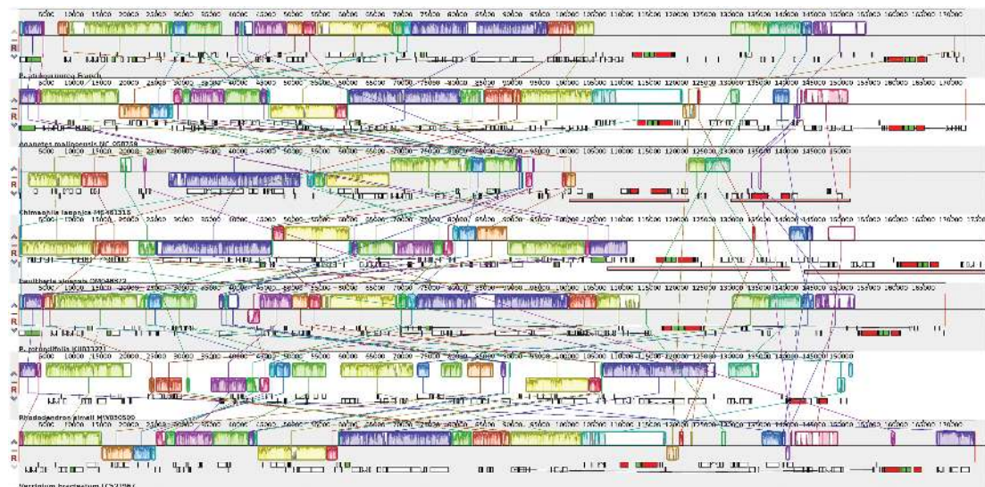
Figure 5: Alignment of chloroplast genomes structure in Ericaceae
