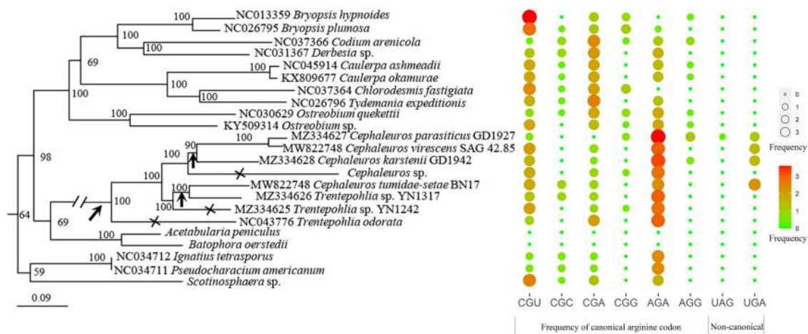
FIGURE 4 | The estimated frequencies of arginine codon usage. Canonical codon AGA is most commonly used, followed by other canonical codon CGU. Among the non-canonical codons, UGA is used more commonly than UAG. (1) A single origin of the non-canonical code along the branch leading to C. parasiticus , C. virescens , C. karstenii , C. tumidae-setae , and Trentepohlia sp. YN1317, and a subsequent reversal to the standard code in Cephaleuros sp., Trentepohlia sp. YN1242, and Trentepohlia odorata (indicated with oblique arrow and cross). (2) A stepwise process of evolution of the non-canonical code with a single initiation of the process along the branch leading to C. parasiticus , C. virescens , C. karstenii , C. tumidae-setae , and Trentepohlia sp. YN1317, followed by a completion of the process in all species except Cephaleuros sp., Trentepohlia sp. YN1242 and Trentepohlia odorata (oblique arrow combined with vertical arrow). (3) Two independent gains of the non-canonical code in the Trentepohliales (vertical arrow).
