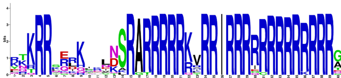
FIGURE 3 | Sequence logo of the position weight matrix reporting the relative amino acid frequencies in the alignment for each abnormal UGA/UAG position in Trentepohliales.
