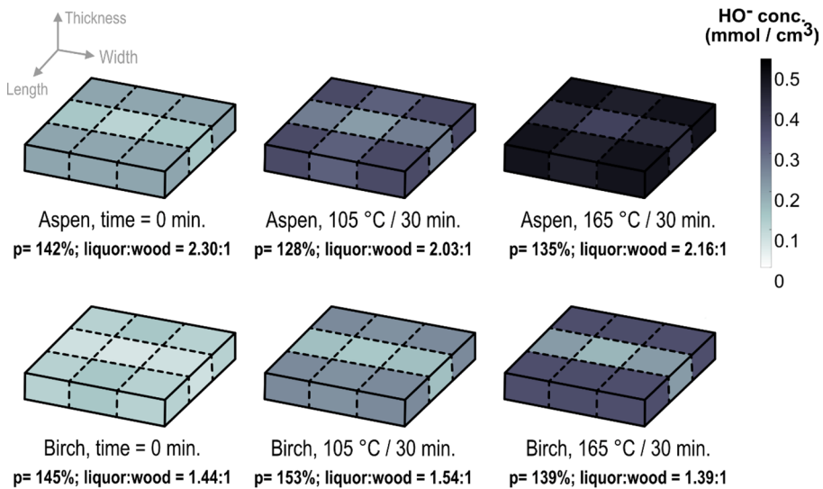
Fig. 2 Degree of liquor penetration ( p ), liquor uptake and distribution of hydroxide ions in wood chips of aspen and birch in three different conditions: after impregnation (20 °C, time = 0 min.), after impregnation and mild treatment (105 °C/30 min), and after impregnation and kraft cooking (165 °C / 30 min). The concentration of hydroxide was measured in different parts of the chips (corners, transverse sides, tangential sides, and center). The results are in mmol of hydroxide ions per volume of impregnated wood (calculated based on measurements of length, width, and thickness) with max. RSD=18%
