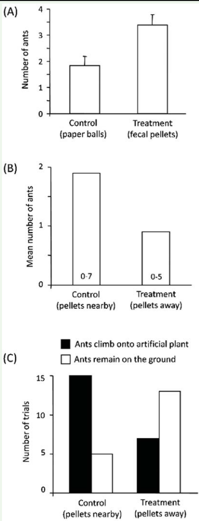
Figure 7. (A) Mean \pm SE number of ants ( Camponotus crassus ) climbing onto an artificial plant after encountering nearby black paper balls and larval fecal pellets ( t = -3.3896 , d.f. = 17, p < 0.01 ). (B) Mean number of ants climbing onto an artificial plant after finding fecal pellets nearby (5 cm) or away (30 cm) from the plant base; numbers inside bars refer to range (Wilcoxon's test, Z = -2.4853 , p < 0.05 ). (C) Proportion of trials in which ants climbed on an artificial plant after finding fecal pellets nearby or away from the plant base ( G = 14.17 , d.f. = 1, p < 0.01 ). High quality figures are available online.
