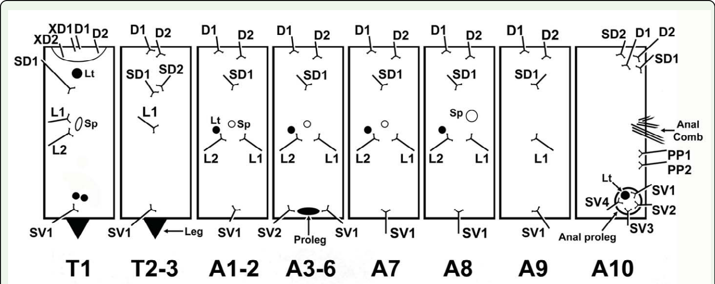
Figure 4. Chaetotaxy of first instar Urbanus esmeraldus . High quality figures are available online.
