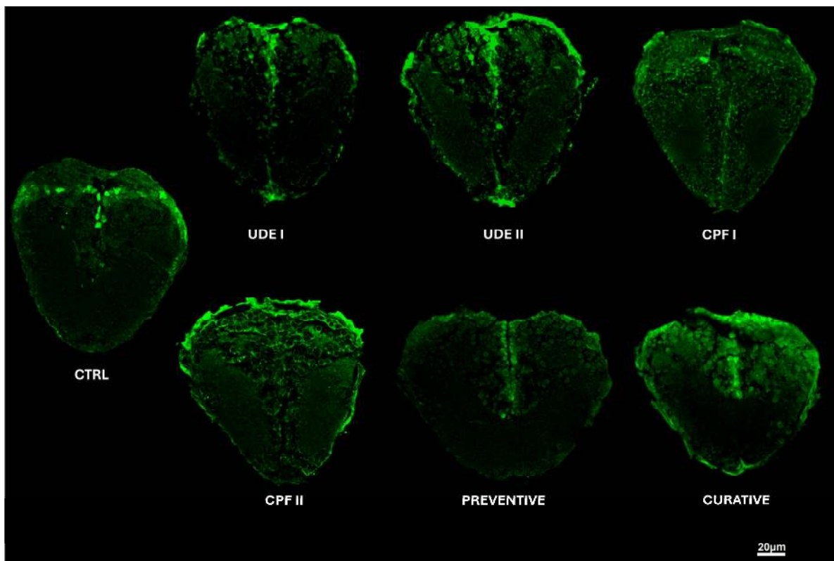
Figure 5. Bdnf immunolabeling in the telencephalon of the control, UDE I, UDE II, CPF I, CPF II, curative, and preventive groups. Scale bar: 20 \mu m.
