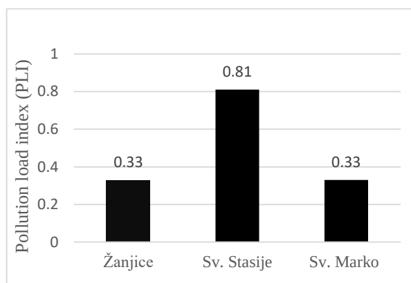
Figure 2. Pollution load index (PLI) for all locations
