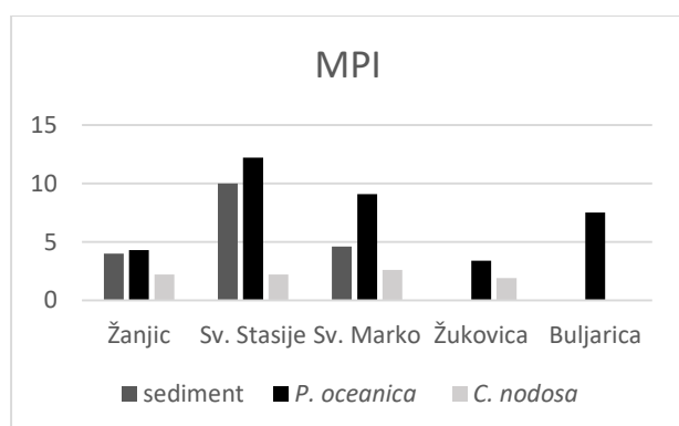
Figure 3. Metal pollution index (MPI) for all location
