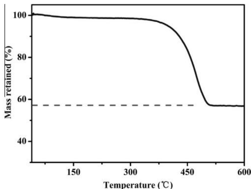
Figure 6: TGA of ZnO nanoparticles
