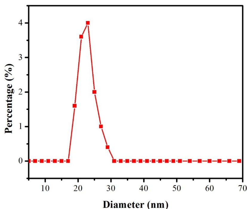
Figure 2: Particle size for ZnO nanoparticles
