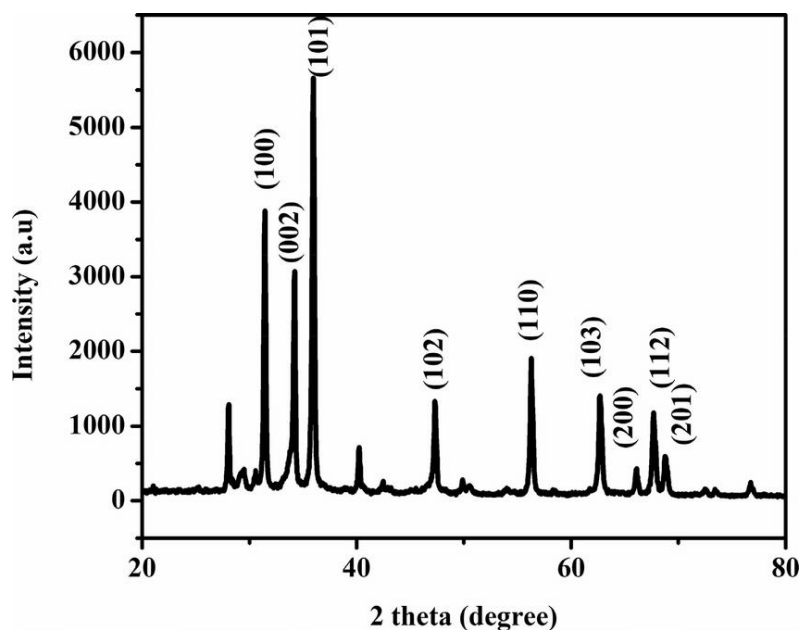
Figure 4. XRD pattern of ZnO nanoparticles.
