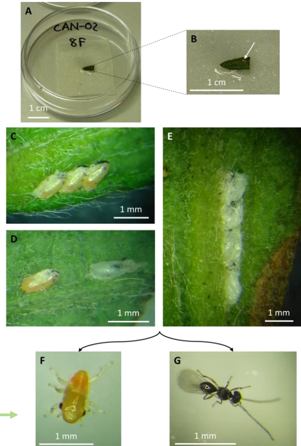
Fig.1 Illustration of the hatching experiment set to identify emerging insects and quantify parasitism rates of Philaenus spumarius
