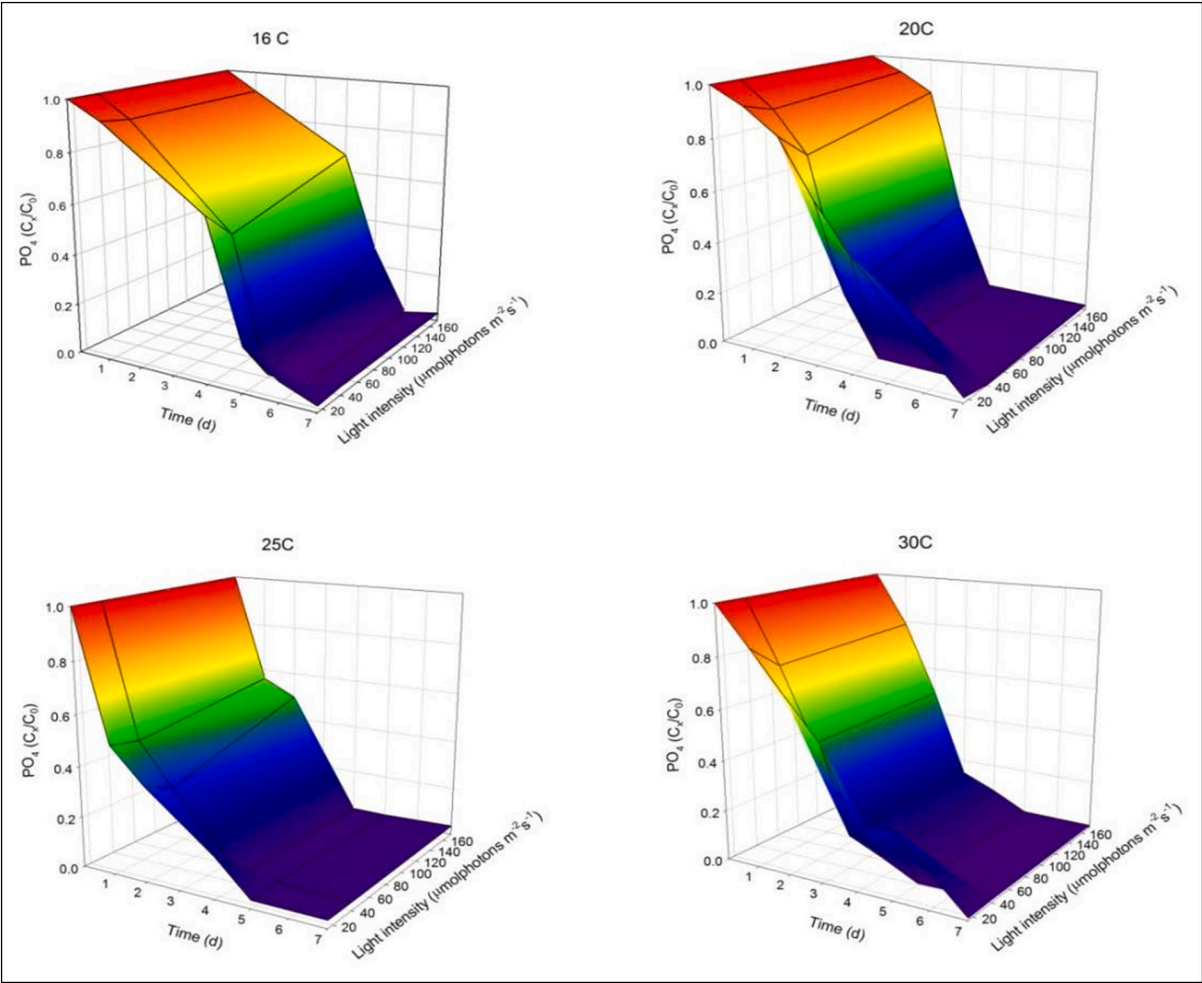
Fig. 2. Removals of \text{PO}_4^{3-} in the medium during incubation at different light intensities and different temperatures, expressed as the ratio between \text{PO}_4^{3-} concentrations in the media ( C_x ) and the initial \text{PO}_4^{3-} concentration ( C_0 ).
