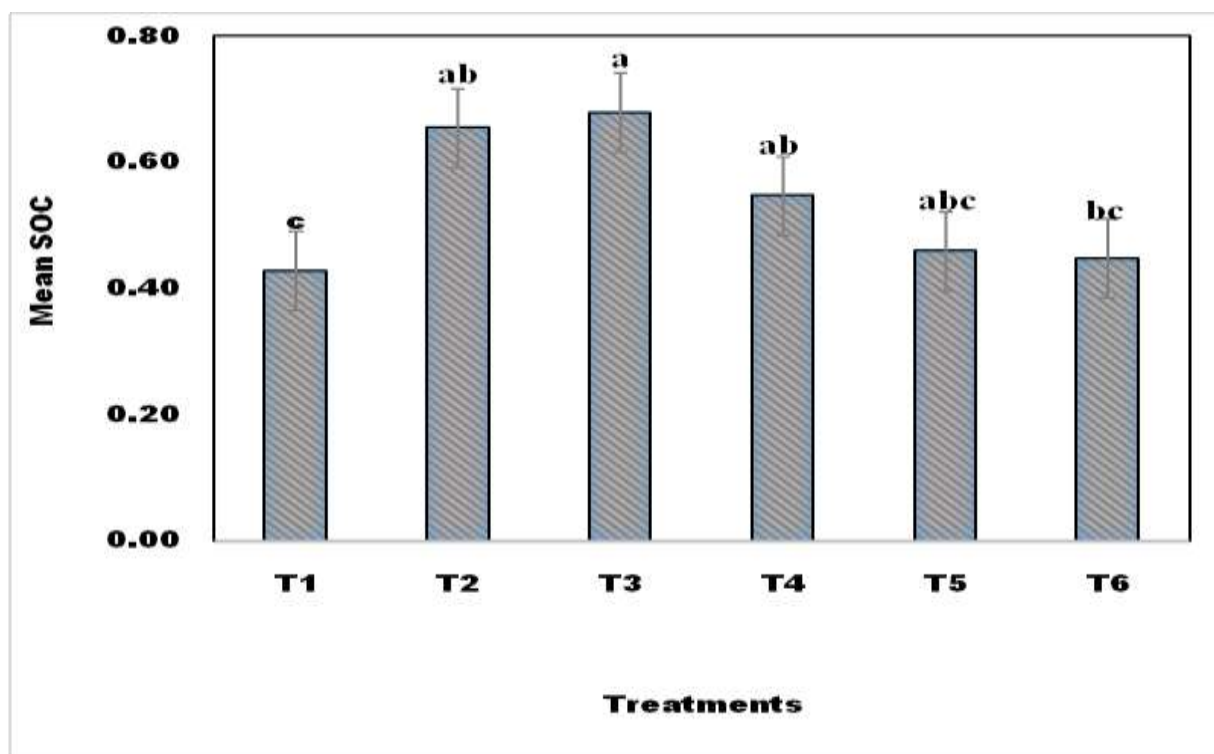
Figure 4: Soil organic carbon as affected by the treatments
