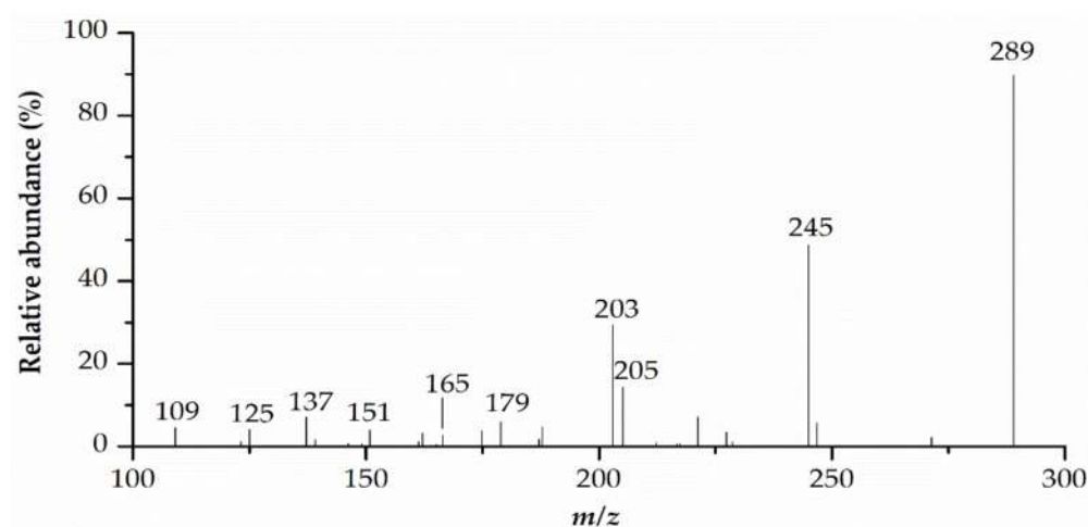
Figure 7. MS/MS spectra for catechin (peak 6). The peak number corresponds to that in Table 2.
