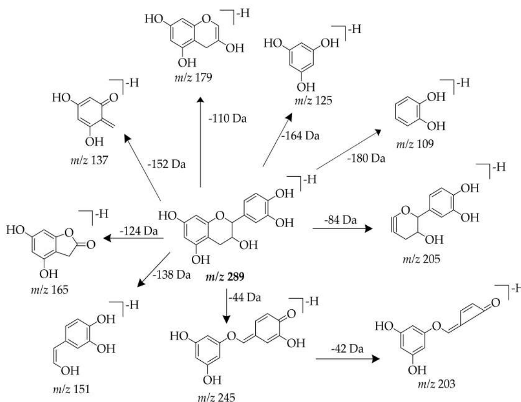
Figure 8. Proposed fragmentation pathway for catechin (peak 6).
