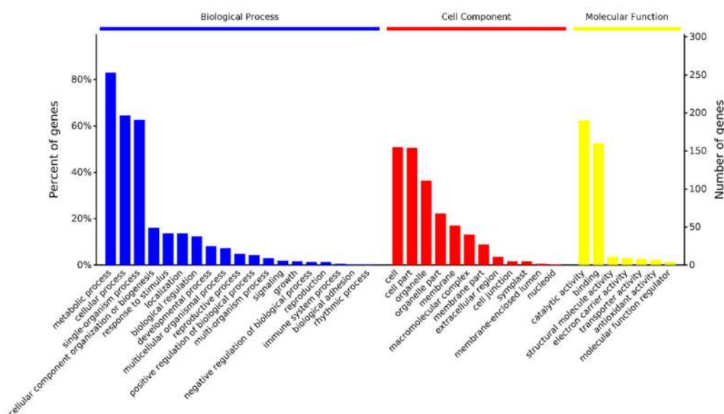
Figure 4. GO functional classification of the identified DAPs.
