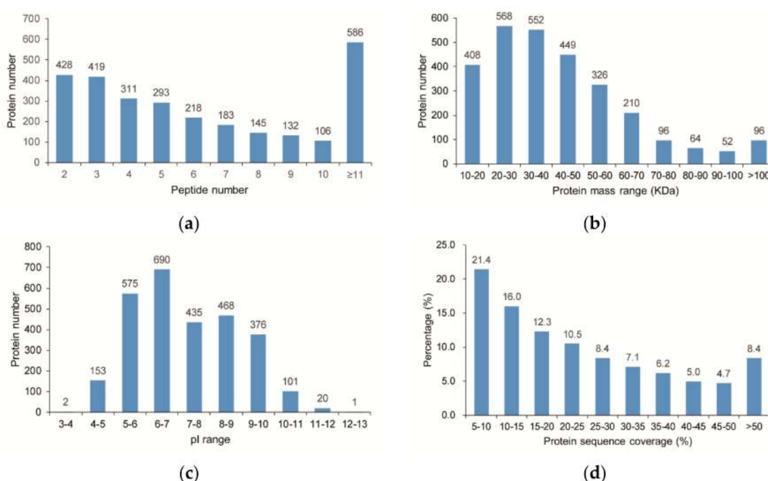
Figure 3. Characteristics of the identified unique proteins in jojoba leaf samples. (a) Unique peptide number distribution; (b) Protein mass distribution; (c) Protein isoelectric point distribution; (d) Peptide coverage of the identified proteins.
