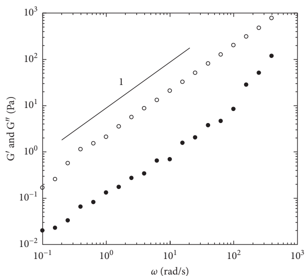
FIGURE 6: Linear viscoelastic properties of small-amplitude oscillatory shear frequency sweep experiment for the jojoba tetraacetate sample at 25°C with 1.0% strain. •: G' ; ○: G'' .
