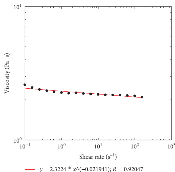
FIGURE 7: The nonlinear viscoelastic properties of the steady shear measurements for the jojoba tetraacetate sample at the temperature of 25°C. Symbols are experiment results; the line is fitted with power law model.
