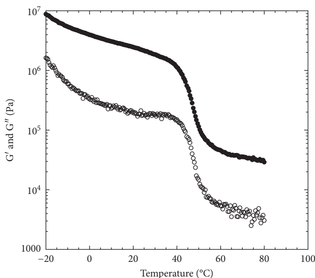
FIGURE 3: The linear viscoelastic properties of aged polyhydroxy jojoba wax with temperature sweep measurement in a range of -20^{\circ}\text{C} to 80^{\circ}\text{C} with the heating rate of 2^{\circ}\text{C}/\text{min} at 1\text{ rad/s} frequency and 0.05\% strain. Filled symbols: G' ; opened symbols: G'' .
