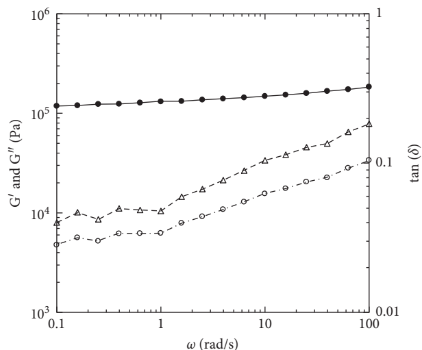
FIGURE 5: Linear viscoelastic properties of small-amplitude oscillatory shear frequency sweep experiment for the aged tetrahydroxy jojoba wax at 70^{\circ}\text{C} with 0.05% strain. ●: G' ; ○: G'' ; △: \tan(\delta) .
