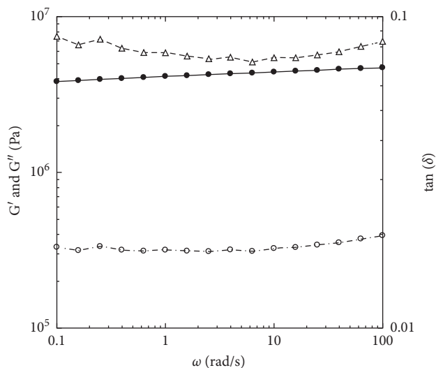
FIGURE 4: Linear viscoelastic properties of small-amplitude oscillatory shear frequency sweep experiment for the aged at 25°C with 0.05% strain. ●: G' ; ○: G'' ; △: \tan(\delta) .
