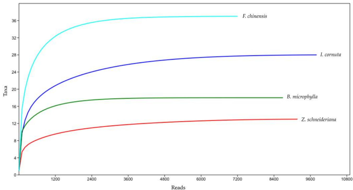
Fig 4. Rarefaction curve of the OTUs from each of the four sampled species.
