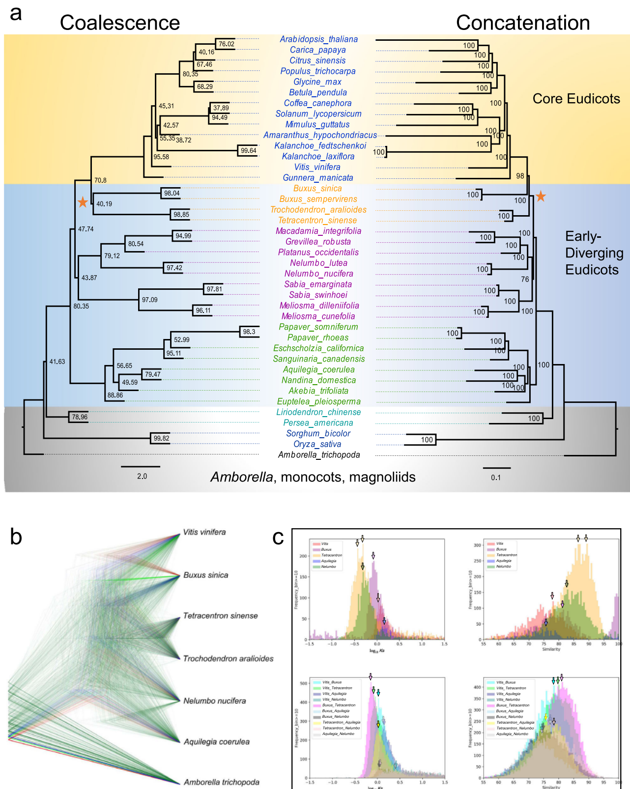
Fig. 2 Phylogenetic relations of Buxus and Tetracentron . a Phylograms depicting the coalescent solution of individual Maximum Likelihood (ML) gene trees (left) and partitioned ML analysis of a supermatrix of nucleotide sequence alignments (right). Node labels indicate quartet (coalescence) and bootstrap (supermatrix) support values, and orange stars highlight the positions of Buxales and Trochodendrales in the two trees. b Cloudogram of 763 SCN gene trees illustrating discordance surrounding the deep branches of eudicot phylogeny. The most frequent trees are blue, the next most frequent red, the third most frequent green, and the rest are dark green. c Ks (left) and Similarity (right) distributions showing peaks (arrows) that stem from WGD (top) and speciation events (bottom), respectively. Source data underlying Fig. 2b, c are provided as a Source data file.
