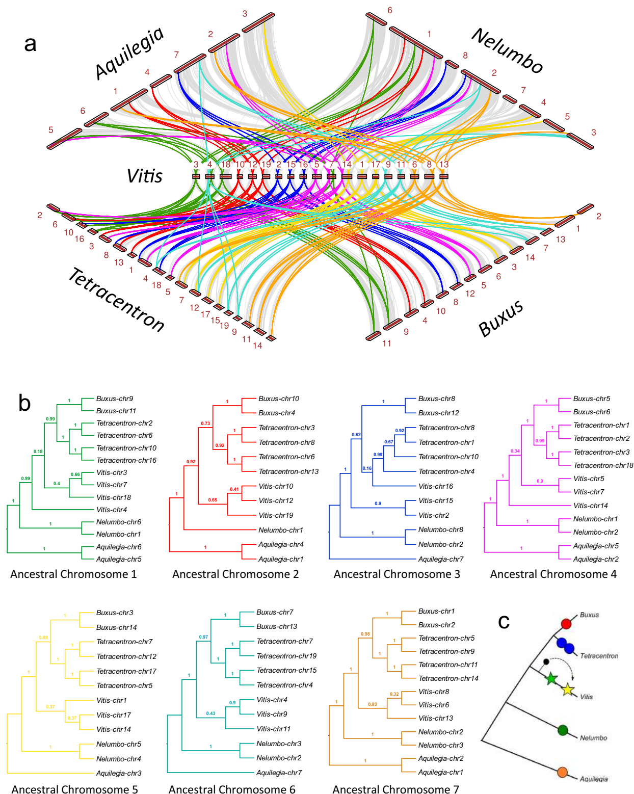
Fig. 3 Synteny and phylogenomics of eudicot subgenomes. a Macrosyntentic alignments of early-diverged eudicots against Vitis with tracking of genomic positions by color-coded syntenic blocks representing the seven ancestral eudicot chromosomes. b Coalescence-based phylogenies of syntenologs derived from duplication events affecting the seven ancestral eudicot chromosomes. Green, red, blue, purple, yellow, aqua, and brown tracks highlight positions of ancestral chromosomes 1 through 7, respectively. Branch labels are posterior probabilities. c Schematic reconstruction of ancient eudicot WGD history. Differently color-filled circles label putative independent duplication events and stars highlight the two gamma WGDs in which the third genome is donated to the initial tetraploid (green star) from an extinct lineage to form the hexaploid (yellow star). Source data underlying Fig. 3a are provided as a Source data file.
