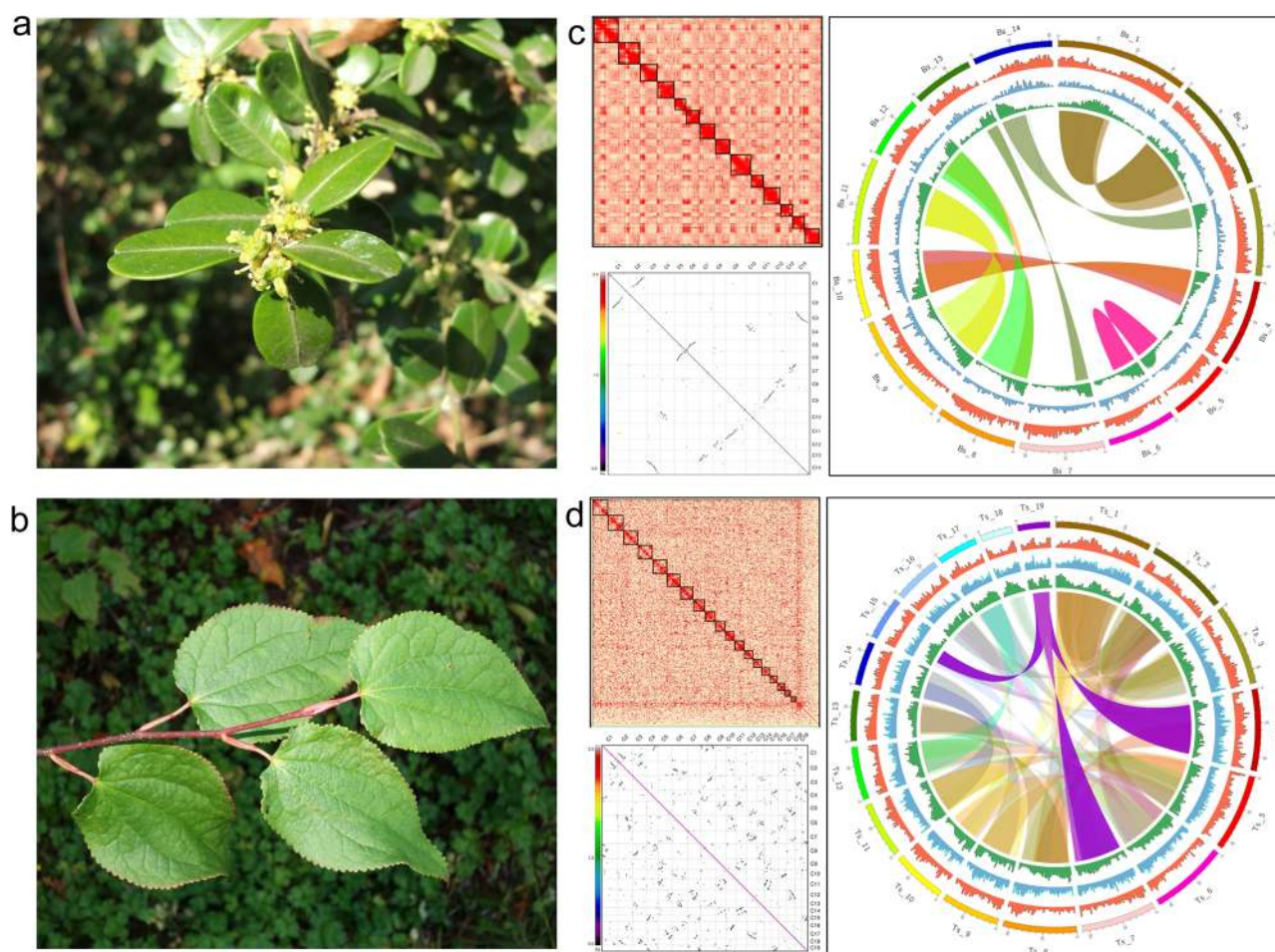
Fig. 1 Habit and genome assembly features of Buxus and Tetracentron . Flowering branch of Buxus sinica ( a ) courtesy of PiPi; and leafy shoot of Tetracentron sinense ( b ) courtesy of Daderot. Hi-C contact heatmaps, intragenomic synteny with syntenic blocks colored according to the Ks scale, and Circos plots for Buxus ( c ) and Tetracentron ( d ). Concentric tracks in the Circos plots, from innermost outwards, show gene, Copia, and Gypsy retrotransposon densities per 1 Mb, and chromosomes, while ribbons connect inter-chromosomal syntenic regions. Source data underlying Fig. 1c, d are provided as a Source data file.
