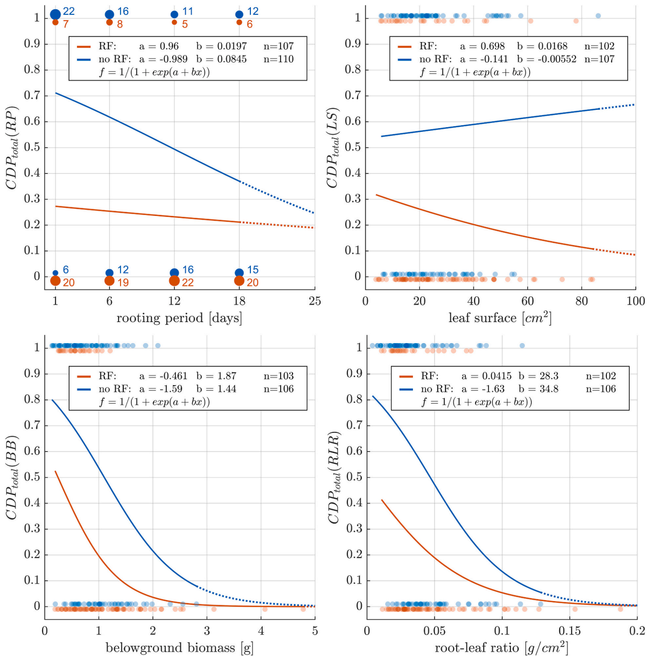
Fig. 8. Binary logistic regression of the influence of the restoration facilitator (RF) on the dislodgement ( CDP_{total} ) as a function of rooting period, leaf surface (LS), the root-leaf ratio ( RLR = BB/LS ) and belowground biomass (BB); Circles indicate binary dislodgement data for each seagrass shoot (0 = not dislodged; 1 = dislodged). Size of Circles in top left plot indicate number of seagrass shoots. Solid lines are the best fit of the function CDP_{total}(RP) = 1/(1 + \exp(a + b(RP))) ; Dotted lines represent the extrapolation of the best fit.
