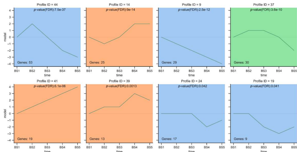
Figure 6. Trend analysis expression module of DEGs. The horizontal axis represents the five periods of flower development, and the vertical axis represents the changes in gene expression at different periods. Different colors indicate different expression patterns ( p \leq 0.05 ).
