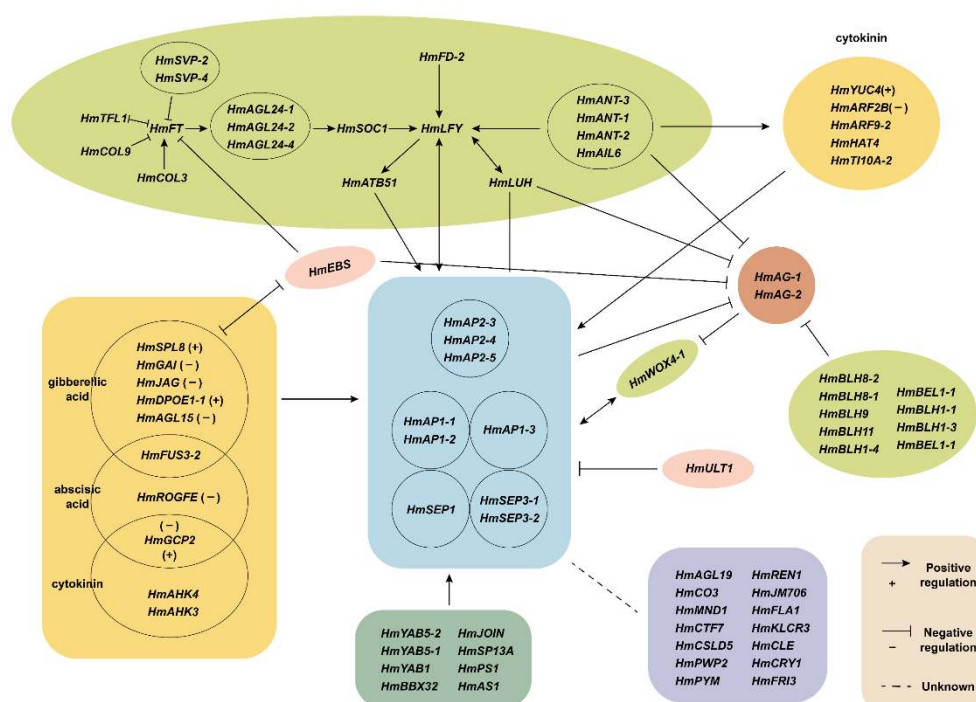
Figure 10. The hypothetical model of gene regulatory network for the development of decorative floret sepals in H. macrophylla .
