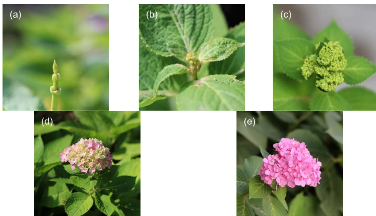
Figure 2. Flower phenotypes at different developmental stages. (a) BS1: vegetative bud, corresponding to Figure 1a. (b) BS2: flower bud, corresponding to Figure 1d. (c) BS3: formation of inflorescence, corresponding to Figure 1f. (d) BS4: initial flowering stage, corresponding to Figure 1k. (e) BS5: full blooming stage, corresponding to Figure 1l.
