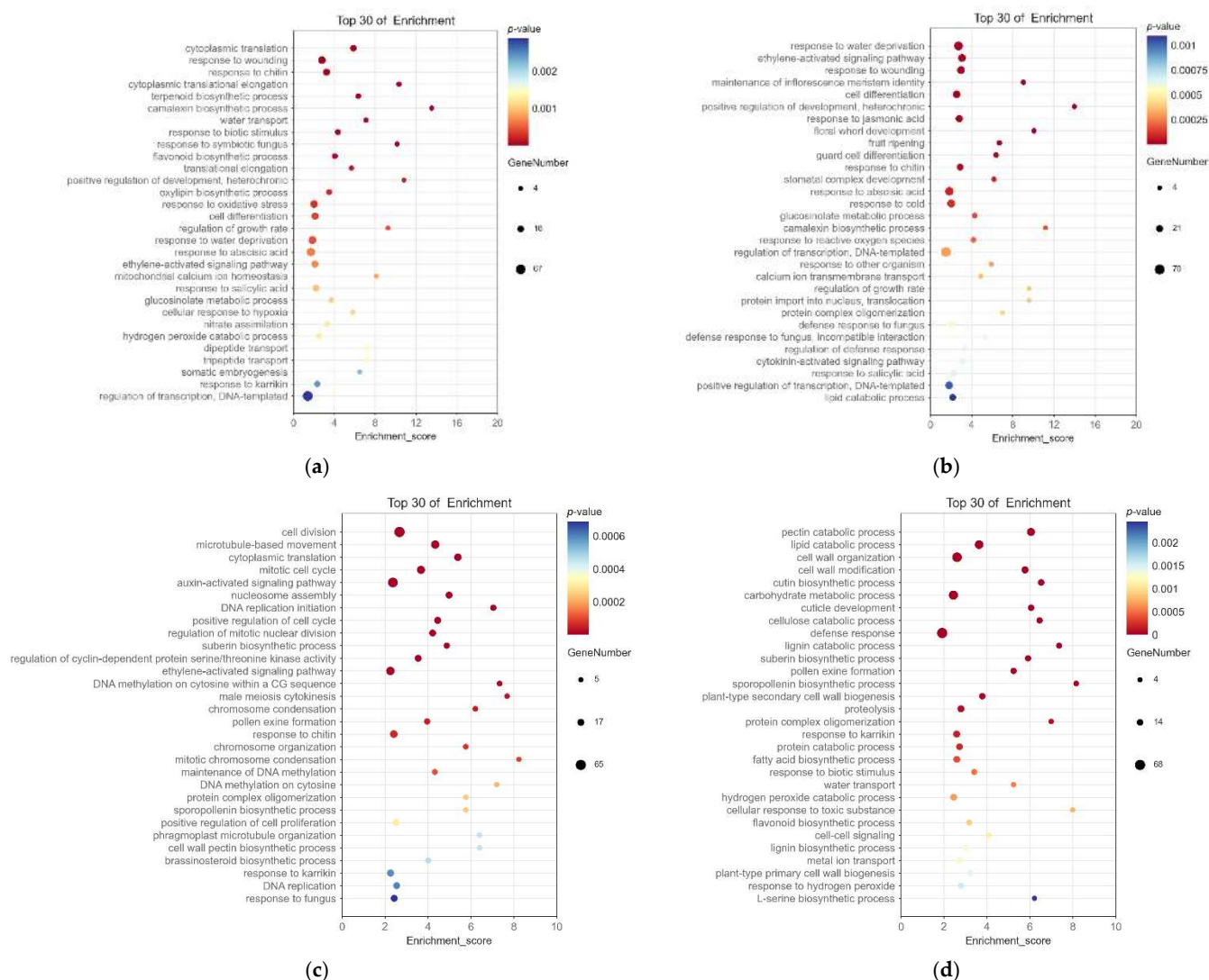
Figure 5. Bubble diagram of the top 30 biological process terms enriched in GO. The horizontal axis in the figure represents the enrichment score, and the vertical axis represents the terms name. The terms with larger bubbles contain a higher number of differential protein-coding genes. The bubble color changes from blue to red, and the smaller the enrichment p -value, the greater the significance. (a) BS1 vs. BS2. (b) BS2 vs. BS3. (c) BS3 vs. BS4. (d) BS4 vs. BS5.
