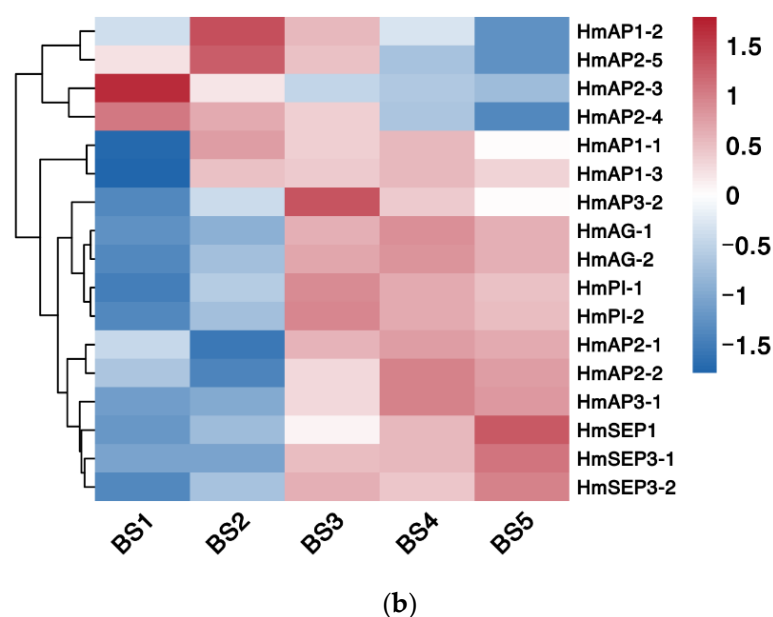
Figure 8. Phylogenetic and expression pattern analysis of genes associated with the ABCDE model. (a) Phylogenetic tree. (b) Cluster heatmap of DEGs related to the ABCDE model. The data preprocessing method takes the logarithm of the sequencing data with 2 as the base. A small square represents a gene, and its color represents the expression level of that gene. Red indicates high-expression genes, and blue indicates low-expression genes. The tree on the left side shows the results of clustering analysis of different genes from different samples.
