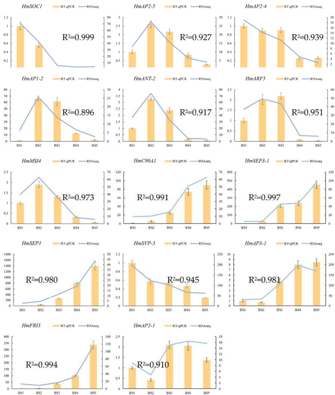
Figure 9. RT-qPCR validation of the expression patterns of 14 DEGs. The x-axis represents the five developmental stages; the left y-axis represents the relative expression levels of RT-qPCR results; the right y-axis represents the FPKM values from RNA-seq. Error bars show the standard error between three biological replicates ( n = 3 ).
