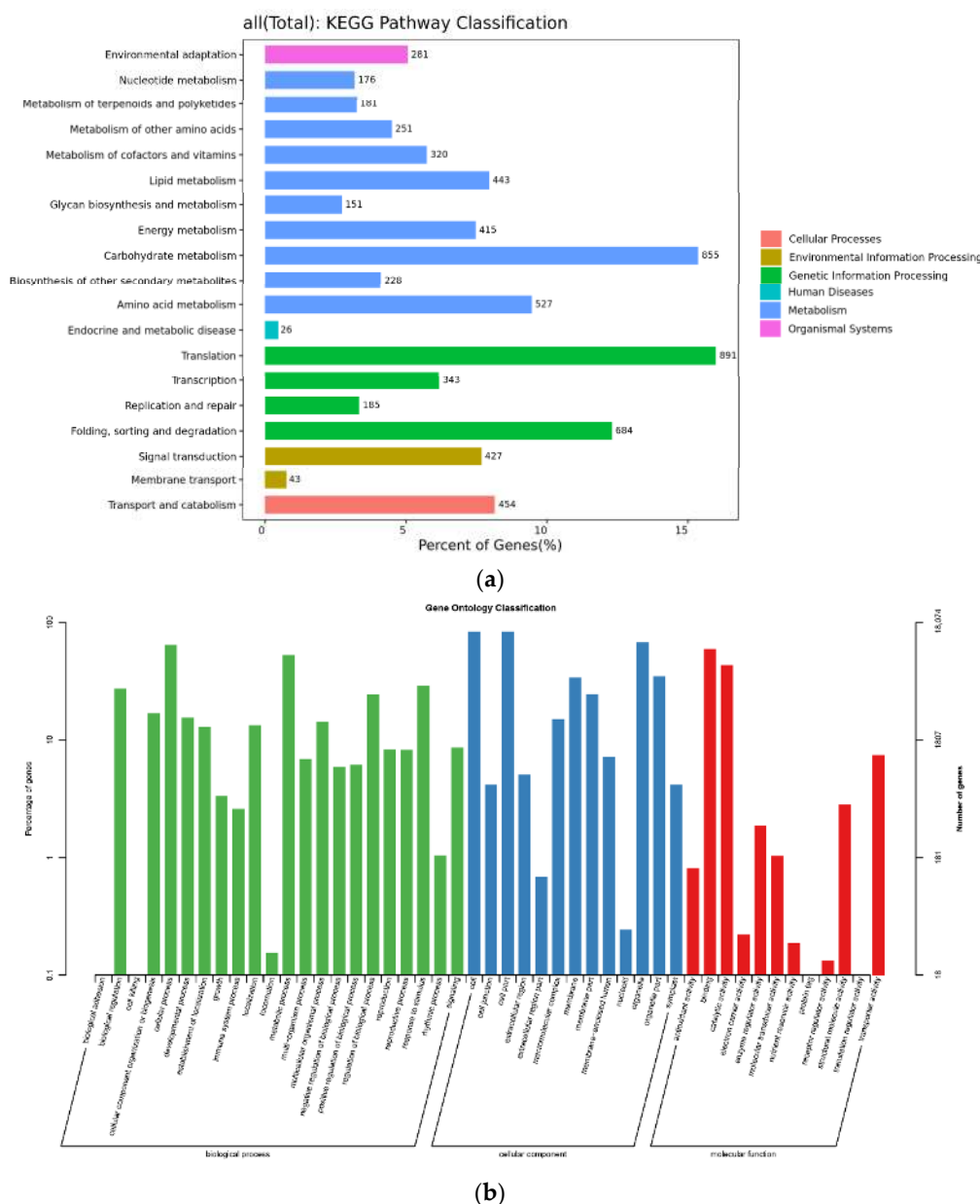
Figure 3. Annotation of unigenes in KEGG and GO datasets. (a) KEGGs. The horizontal axis represents the percent of genes annotated to the pathway; the vertical axis represents the Level 2 pathway name, and the number on the right of the bar represents the number of genes annotated to this Level 2 pathway. (b) GO. The horizontal axis represents the GO functional classification; the left vertical axis represents the percentage of genes annotated to that class, and the right vertical axis represents the number of genes annotated to that class.
