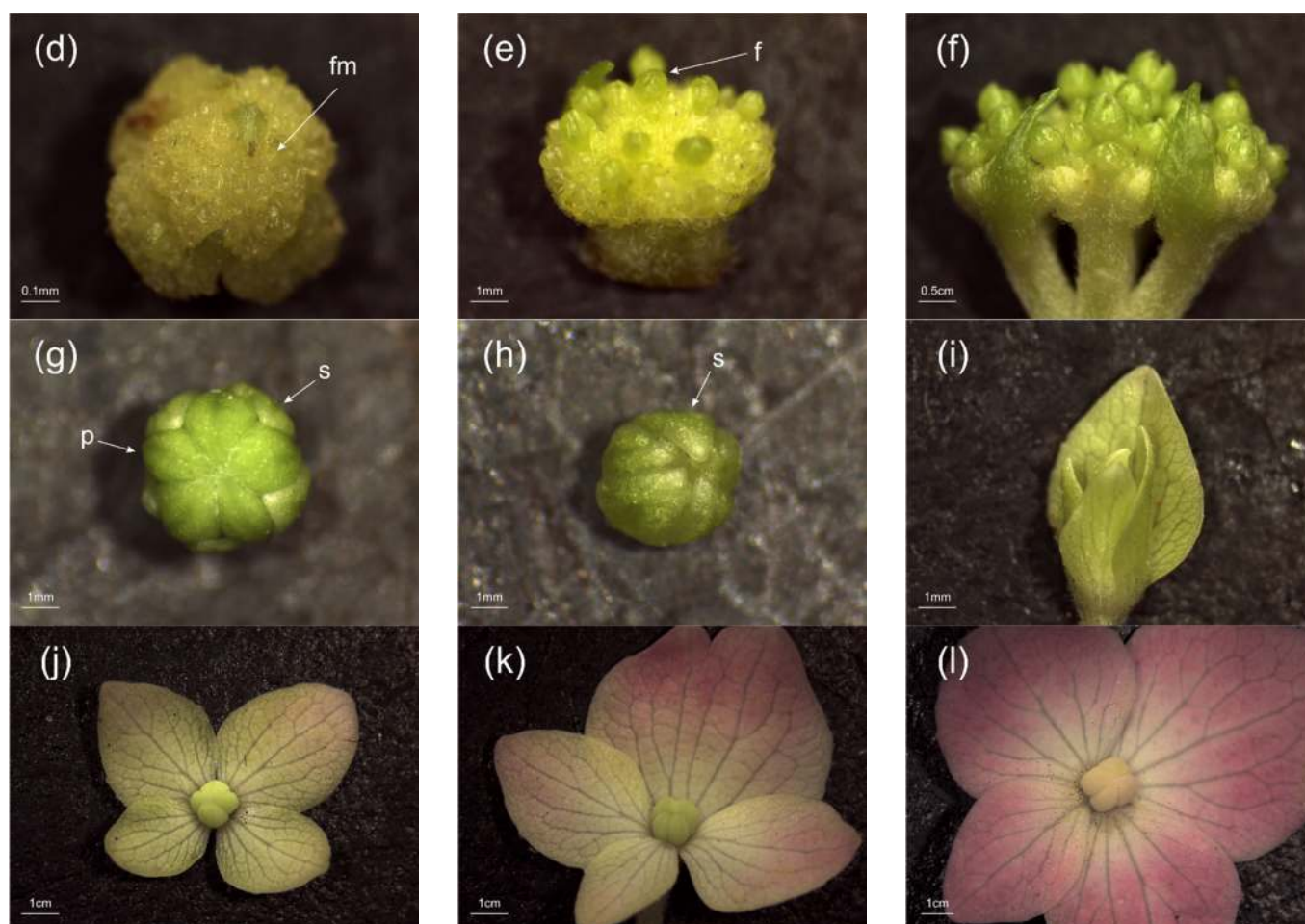
Figure 1. Flower development stages of Hydrangea macrophylla 'Endless Summer' observed by stereomicroscope. (a) Vegetative bud. (b) Inflorescence meristem dome formation begins. (c) Spherical shape formed by numerous inflorescence meristem domes. (d) Floral primordium differentiation stage. (e) Floral organ differentiation stage. (f) Secondary branching of spherical inflorescence. (g) Nondecorative floret on secondary inflorescence branching. (h) Decorative floret on secondary inflorescence branching. (i) Decorative floret with elongated sepals. (j) Decorative floret sepals unfold. (k) Decorative floret sepals start to turn color. (l) Decorative floret sepals completely changed color. vm = vegetative meristem; im = inflorescence meristem; fm = floral meristem; fp = foliar primordia; f = floret; s = sepal; p = petal.
