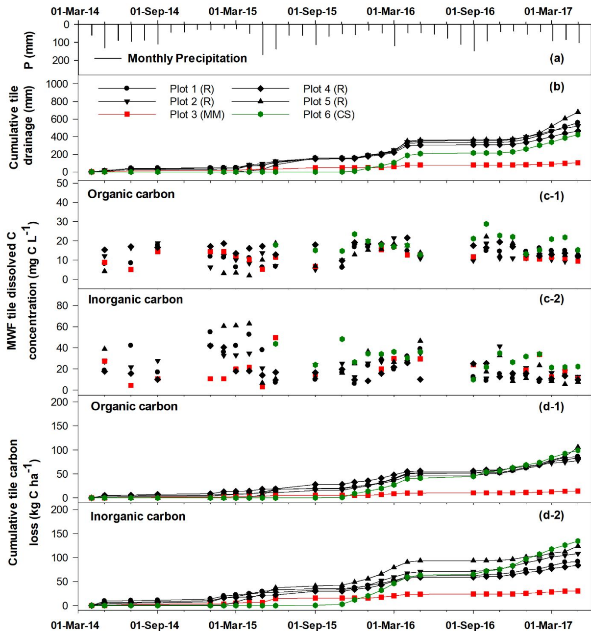
Figure 2. Monthly precipitation (a), cumulative tile drainage (b), flow-weighted mean dissolved organic and inorganic carbon concentrations in tile drainage water (c-1 and c-2), and cumulative loss of dissolved organic and inorganic carbon in tile drainage (d-1 and d-2) from May 2014 to May 2017. Treatments included monoculture maize (MM), continuous Kentucky blue grass sod (CS) and a 4-yr alfalfa-alfalfa-maize-oat rotation with each phase present each year (R).
