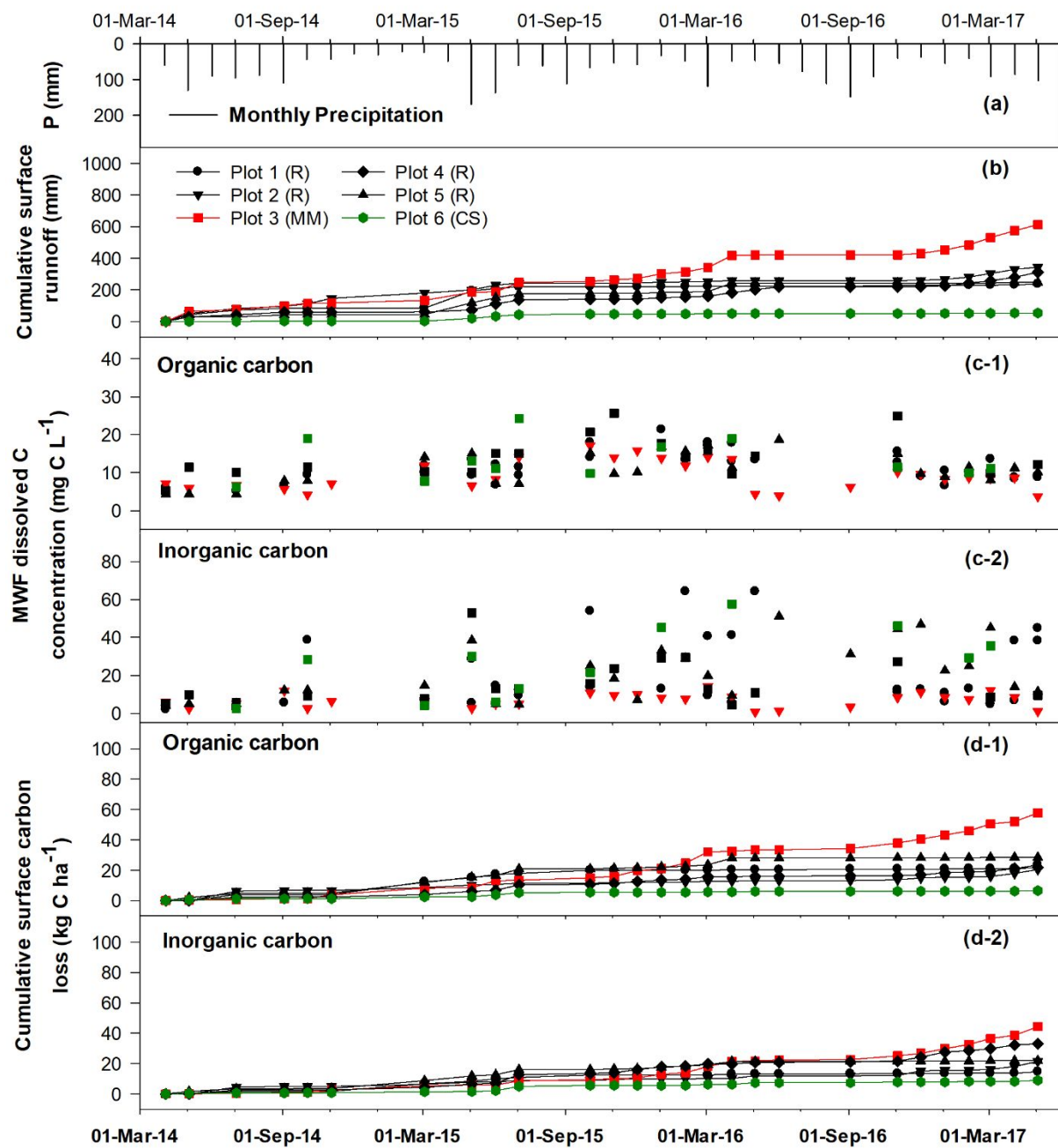
Figure 3. Monthly precipitation (a), cumulative surface runoff (b), flow-weighted mean dissolved organic and inorganic carbon concentrations in surface runoff (c-1 and c-2), and cumulative loss of dissolved organic and inorganic carbon in surface runoff (d-1 and d-2) from May 2014 to May 2017. Treatments included monoculture maize (MM), continuous Kentucky blue grass sod (CS) and a 4-yr alfalfa-alfalfa-maize-oat rotation with each phase present each year (R).
