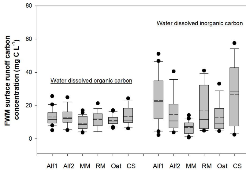
Figure 5. Flow weighted mean (FWM) dissolved organic and inorganic carbon concentrations in surface runoff water collected from May 2014 to May 2017. Treatments included a first year alfalfa (Alf1), second year alfalfa (Alf2), monoculture maize (MM), rotation maize (RM), oat (Oat), and continuous Kentucky blue grass sod (CS). Boxes indicate the 25 th and 75 th percentile, T-bars above and below the box indicate the 90 th and 10 th percentile, solid dots indicate outliers, dashed lines indicate mean, and solid lines indicate median.
