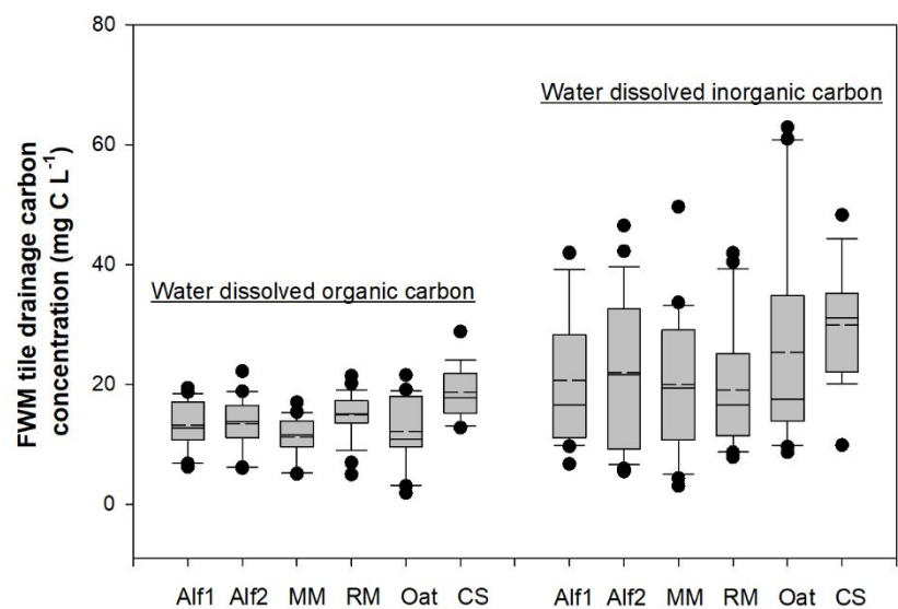
Figure 4. Flow weighted mean (FWM) dissolved organic and inorganic carbon concentrations in tile drainage water collected from May 2014 to May 2017. Treatments included a first year alfalfa (Alf1), second year alfalfa (Alf2), monoculture maize (MM), rotation maize (RM), oat (Oat), and continuous Kentucky blue grass sod (CS). Boxes indicate the 25 th and 75 th percentile, T-bars above and below the box indicate the 90 th and 10 th percentile, solid dots indicate outliers, dashed lines indicate mean, and solid lines indicate median.
