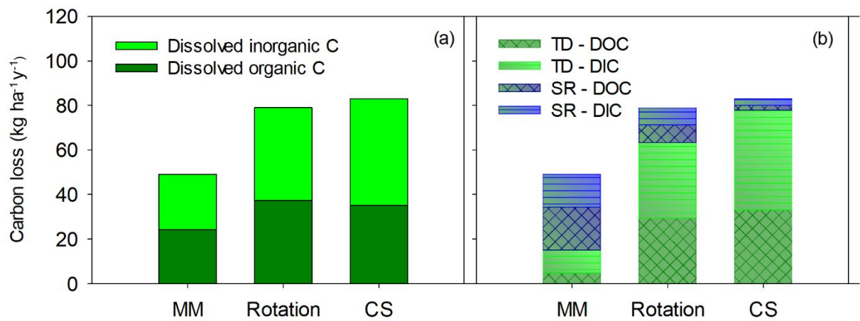
Figure. 6. Partitioning of total carbon loss from monoculture maize (MM), continuous Kentucky blue grass sod (CS), and an alfalfa-alfalfa-maize-oat rotation (Rotation) between: a) dissolved organic and inorganic carbon; b) tile drainage and surface runoff.
