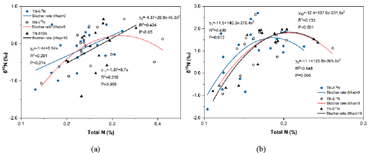
Fig. 3 Non-linear relationship between soil total nitrogen (N) and soil \delta^{15}\text{N} (‰) of three biochar rates (0, 5 and 10 t/ha) at soil depth of 0–5 cm (a) and 5–10 cm (b) respectively
