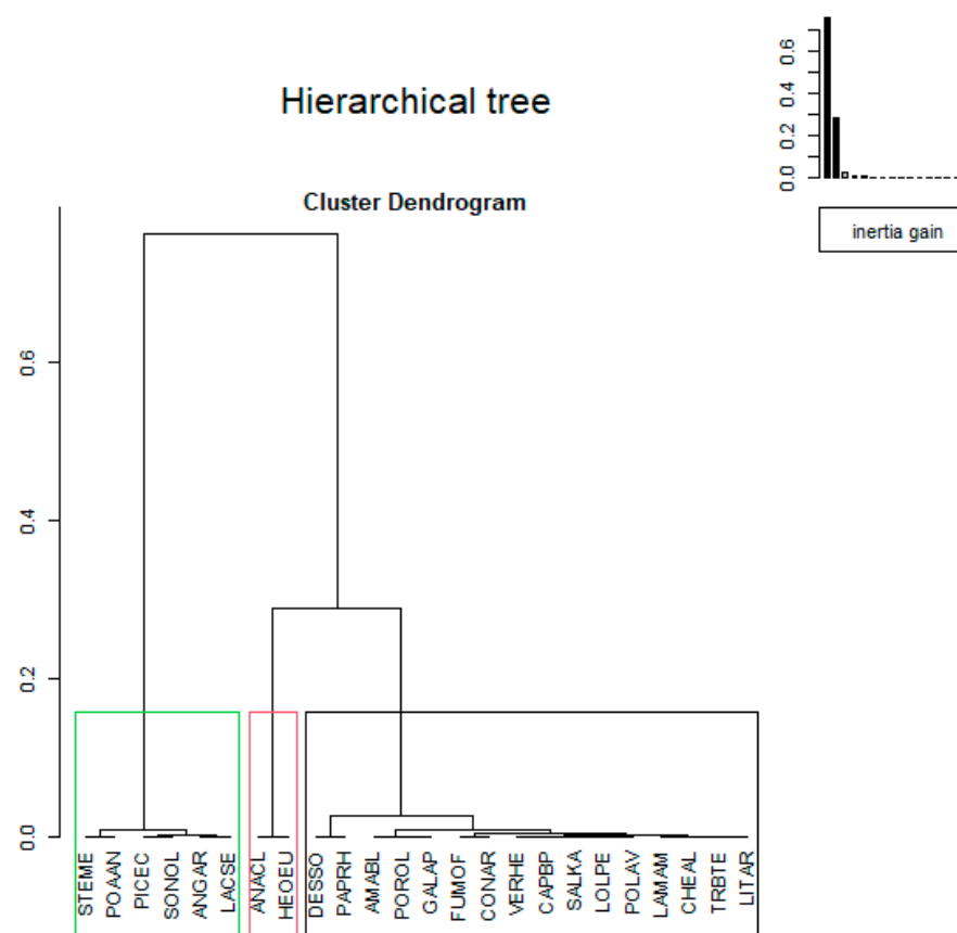
Figure 4. Plots graphs from a HCPC result: hierarchical tree. The dendrogram suggests a three clusters solution. In this tree visualize individuals (weed species) on the principal component map and to color individuals according to the cluster they belong to: Black: M site-extraction-2018, 2019, 2020; Red: M site-germination-2020 and Green: S site-extraction and germination-2018, 2019, 2020.
