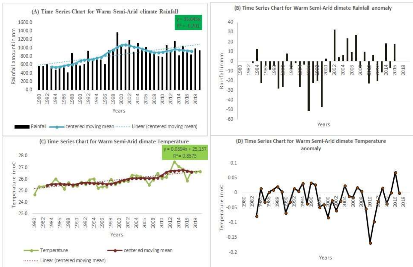
Figure 5: Rainfall and Temperature time series and anomaly plots for the Warm Semi-Arid Climate Belt.
