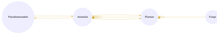
Figure 3: Interactions on taxonomic kingdom rank as interpreted by the Catalogue of Life download svg
