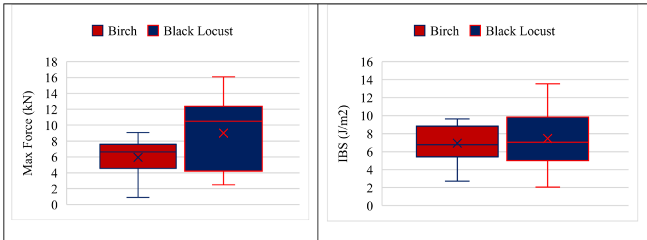
Fig. 6 Max inflicted force and the IBS of the species
