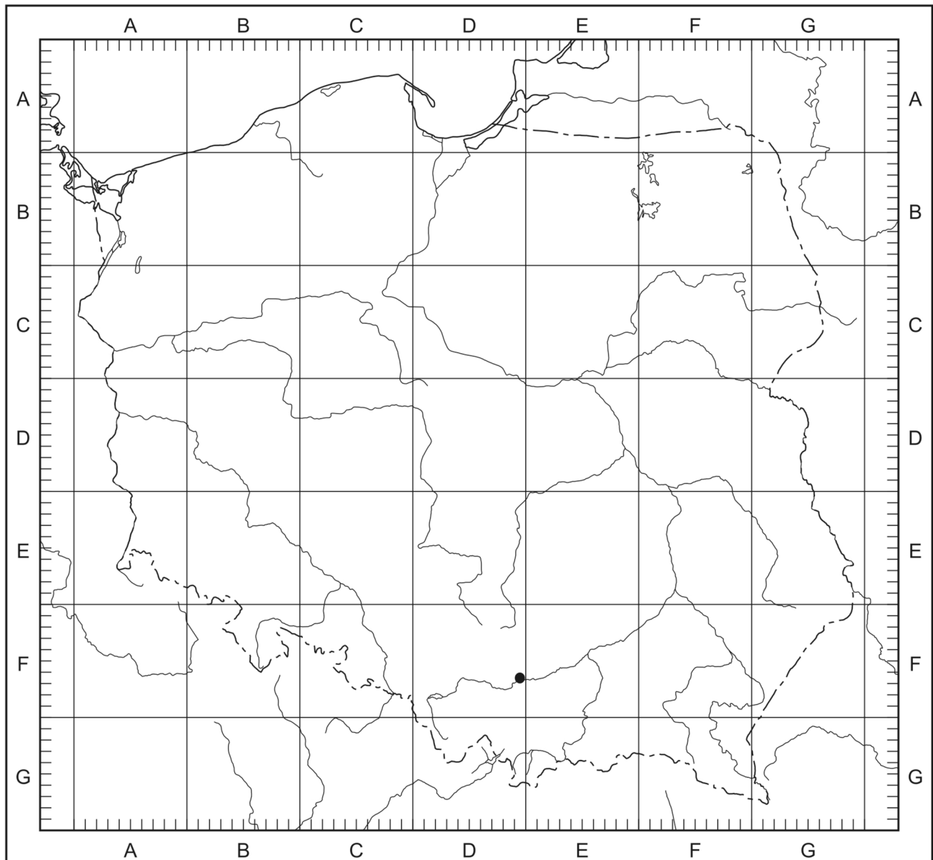
Fig. 4 Locality (black dot) of Ludwigia repens and Myriophyllum aquaticum in Poland within the ATPOL cartogram grid
