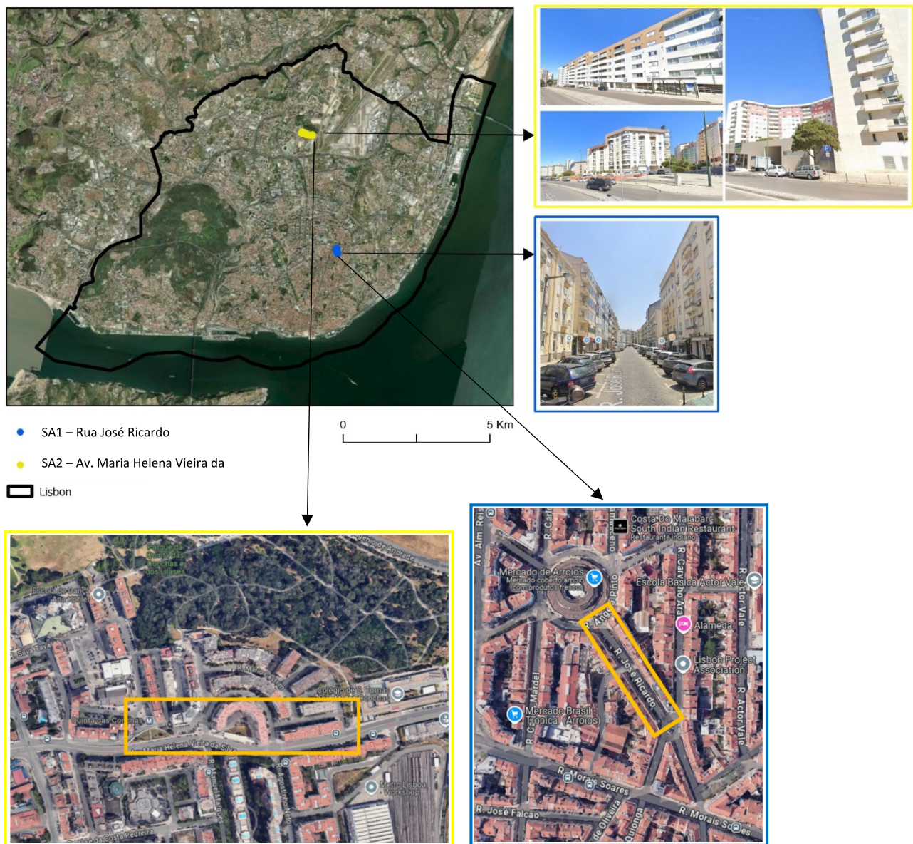
Fig. 1 Envi-met simulation areas. The orange boxes in the satellite images are the area of interest for the simulations
