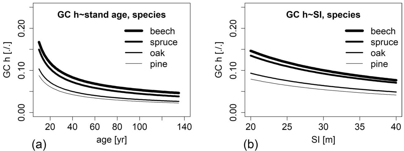
Fig. 4 Effect of stand age and site index on the vertical structural diversity GCh of unthinned stands (A-grade) of European beech, Norway spruce, sessile/common oak, and Scots pine. Visualization of the
