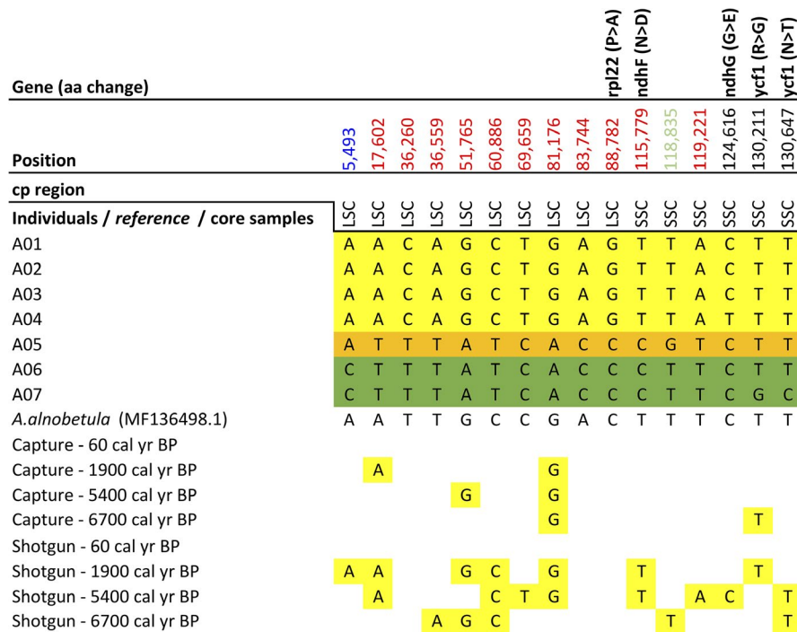
FIGURE 5 Single-nucleotide polymorphisms (SNPs) detected in the whole chloroplast genome alignment of the seven Alnus alnobetula individuals. The reference chloroplast genome and the sedaDNA retrieved from core samples through hybridization capture and shotgun sequencing methods were mapped subsequently in order to evaluate their variants corresponding to the SNPs' positions. An SNP's position corresponds to the reference chloroplast genome. If an SNP is located within a gene, the corresponding gene name is given in the first row. If no reads were retrieved from core samples, no variant is reported. Color code: Taymyr specific variation = yellow; Omoloy specific variation = orange; Kolyma specific variation = green; potential marker for Taymyr geographic discrimination = position highlighted in red; potential marker for Kolyma geographic discrimination = position highlighted in blue; potential marker for Omoloy geographic discrimination = position highlighted in light green
