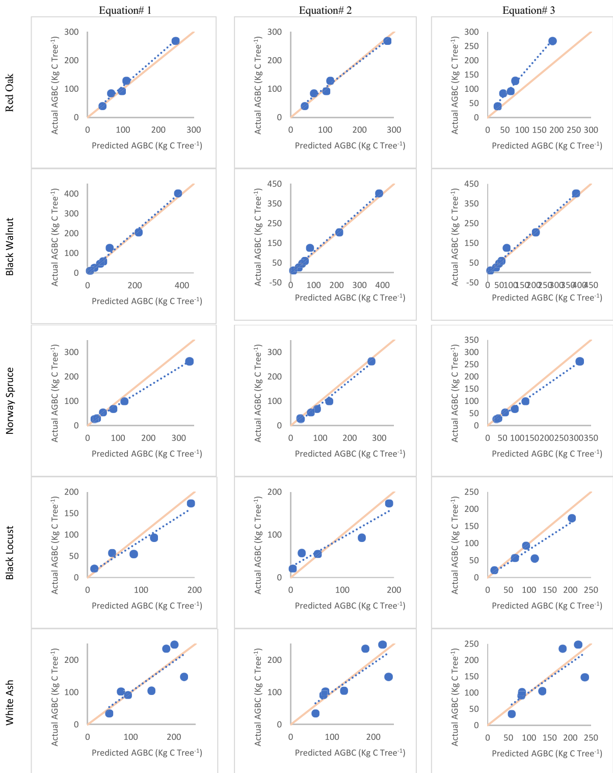
Fig. 2 Comparison of predicted C sequestration by equations nos. 1–3 in five tree species under tree-based intercropping systems and observed C sequestration in aboveground bio-
