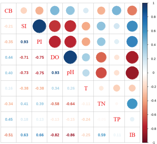
Figure 7. Correlations of the community indicators and physical and chemical water properties with invasive plants. Pairwise correlations of these variables are shown with a color gradient denoting Pearson’s correlation coefficients. CB denotes “community total biomass”; SI denotes “Shannon-Wiener diversity index”; PI means “Pielou evenness index”; DO denotes “dissolved oxygen”; T denotes “transparency”; TN denotes “total nitrogen content”; TP means “total phosphorus content”; IB denotes “invasion plant biomass.”
