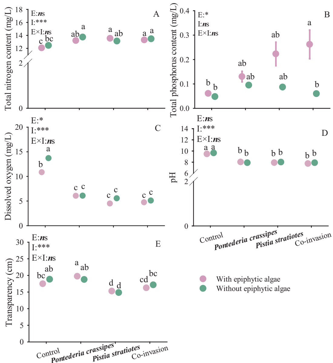
Figure 6. Effects of invasion scenarios (I) and epiphytic algae (E) on Physical and Chemical Properties of Water (mean + SE, n = 5 ). Control denotes “no invasion”; Pontederia crassipes denotes “ Pontederia crassipes invasion”; Pistia stratiotes denotes “ Pistia stratiotes invasion”; co-invasion denote “co-invasion of Pontederia crassipes and Pistia stratiotes ”; * denotes “ P < 0.05 ”; *** denotes “ P < 0.001 .” Different letters indicate significant differences among treatments ( P < 0.05 ).
