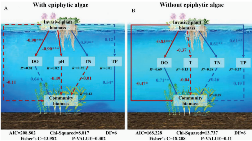
Figure 8. Structural equation modeling diagram of the relationship between the invasive plants, physical and chemical water properties, and community biomass. Rectangles represent measurable variables, and single arrows represent path coefficients; solid lines indicate significant effects ( P < 0.05 ), dashed lines indicate non-significant effects, blue lines denote positive effects, red lines denote negative effects, * means P < 0.05 , ** means P < 0.01 , *** means P < 0.001 . DO: dissolved oxygen; TN: total nitrogen content; TP: total phosphorus content; T: transparency.
