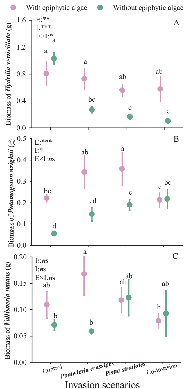
Figure 2. Effects of invasion scenarios (I) and epiphytic algae (E) on biomass of three submerged plants (mean + SE, n = 5 ). Control denotes “no invasion”; Pontederia crassipes denotes “ Pontederia crassipes invasion”; Pistia stratiotes denotes “ Pistia stratiotes invasion”; co-invasion denote “co-invasion of Pontederia crassipes and Pistia stratiotes ”; * denotes “ P < 0.05 ”; ** denotes “ P < 0.01 ”; *** denotes “ P < 0.001 .” Different letters indicate significant differences among treatments ( P < 0.05 ).
