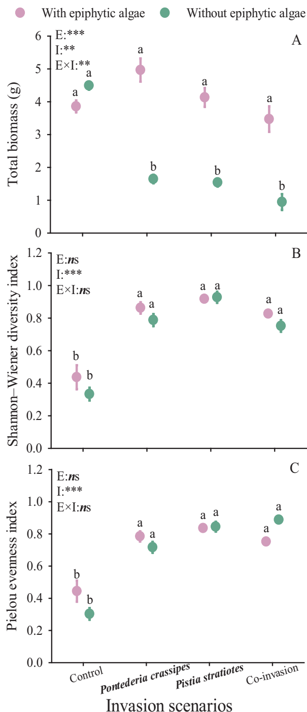
Figure 3. Effects of invasion scenarios (I) and epiphytic algae (E) on indicators of submerged plant communities (mean + SE, n = 5 ). Control denotes “no invasion”; Pontederia crassipes denotes “ Pontederia crassipes invasion”; Pistia stratiotes denotes “ Pistia stratiotes invasion”; co-invasion denote “co-invasion of Pontederia crassipes and Pistia stratiotes ”; ** denotes “ P < 0.01 ”; *** denotes “ P < 0.001 .” Different letters indicate significant differences among treatments ( P < 0.05 ).
