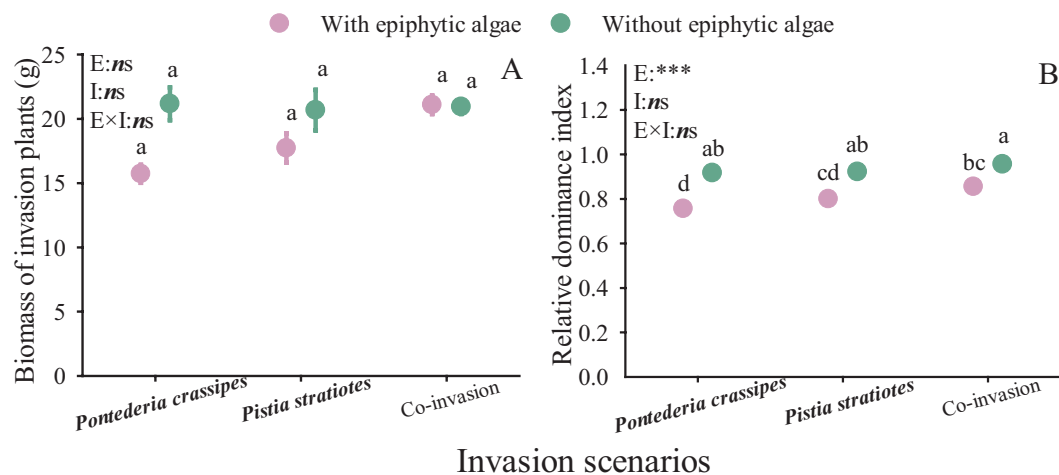
Figure 5. Effects of invasion scenarios (I) and epiphytic algae (E) on biomass and relative dominance index of invasion plants (mean + SE, n = 5 ). Pontederia crassipes denotes “ Pontederia crassipes invasion”; Pistia stratiotes denotes “ Pistia stratiotes invasion”; co-invasion denotes “co-invasion of Pontederia crassipes and Pistia stratiotes ”; *** denotes “ P < 0.001 .” Different letters indicate significant differences among treatments ( P < 0.05 ).
